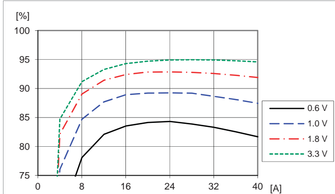
Efficiency vs. load current and output voltage at T_{P1} = +25\text{ }^\circ\text{C} , V_i = 12\text{ V} , f_{sw} = 320\text{ kHz} , C_0 = 470\text{ }\mu\text{F}/10\text{ m}\Omega .
