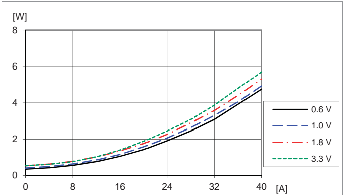
Dissipated power vs. load current and output voltage: T_{P1} = +25\text{ }^\circ\text{C} , V_i = 5\text{ V} , f_{sw} = 320\text{ kHz} , C_0 = 470\text{ }\mu\text{F}/10\text{ m}\Omega .
