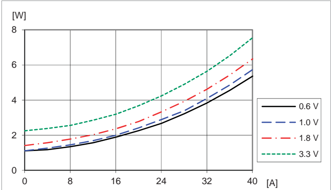
Dissipated power vs. load current and output voltage: T_{P1} = +25\text{ }^\circ\text{C} , V_i = 12\text{ V} , f_{sw} = 320\text{ kHz} , C_0 = 470\text{ }\mu\text{F}/10\text{ m}\Omega .
