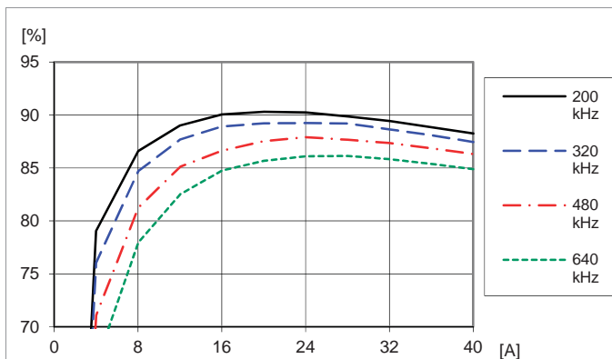
Efficiency vs. load current and switch frequency at T_{P1} = +25\text{ }^\circ\text{C} , V_i = 12\text{ V} , V_o = 1.0\text{ V} , C_0 = 470\text{ }\mu\text{F}/10\text{ m}\Omega Default configuration except changed frequency
