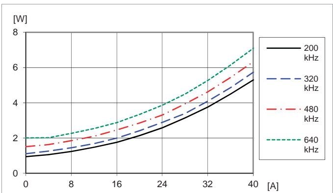
Dissipated power vs. load current and switch frequency at T_{P1} = +25\text{ }^\circ\text{C} , V_i = 12\text{ V} , V_o = 1.0\text{ V} , C_0 = 470\text{ }\mu\text{F}/10\text{ m}\Omega Default configuration except changed frequency
