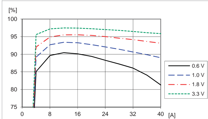
Efficiency vs. load current and output voltage: T_{P1} = +25\text{ }^\circ\text{C} , V_i = 5\text{ V} , f_{sw} = 320\text{ kHz} , C_0 = 470\text{ }\mu\text{F}/10\text{ m}\Omega .
