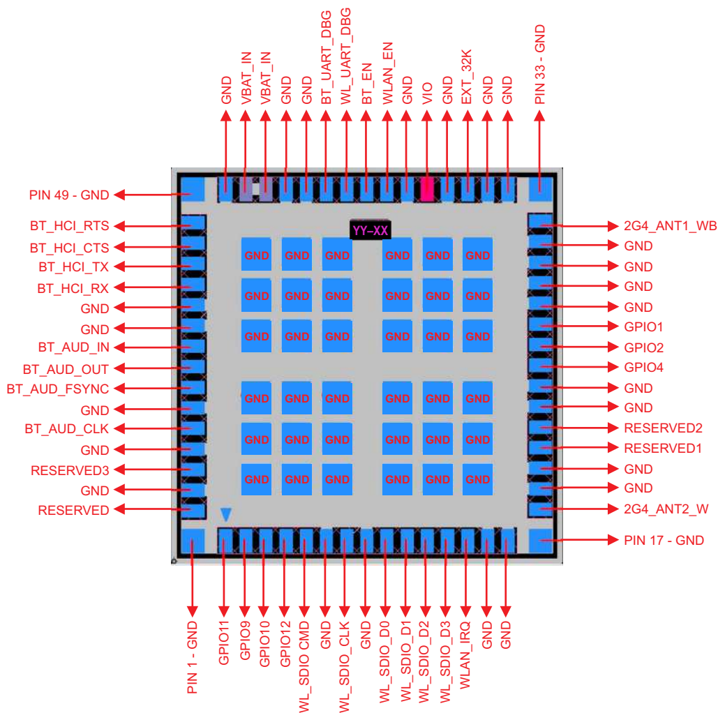
Figure 4-1. 100-Pin MOC Package (Bottom View)
