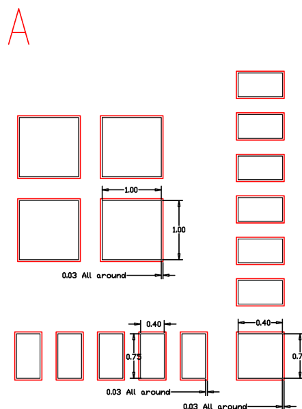
Figure 4-3. Outline of Recommended PCB Pattern for 100-Pin MOC Package (Bottom View)
