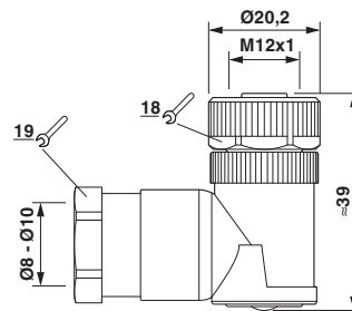
Dimensioned drawing
