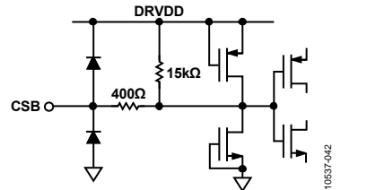
Figure 49. Equivalent CSB Input Circuit
