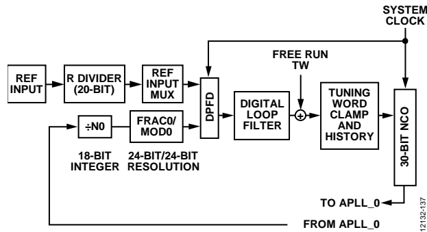
Figure 27. DPLL_0 Core
