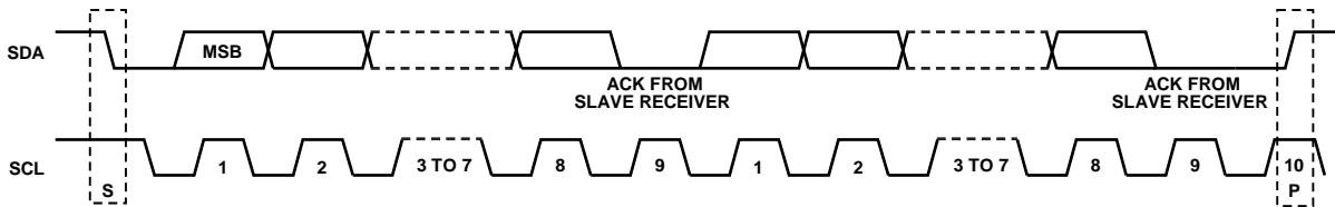
Figure 41. Acknowledge Bit
