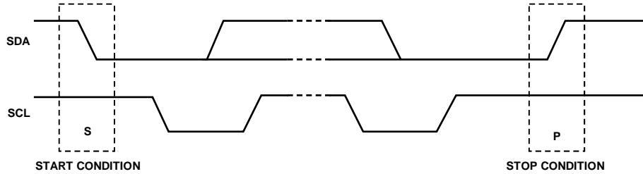
Figure 40. Start and Stop Conditions
