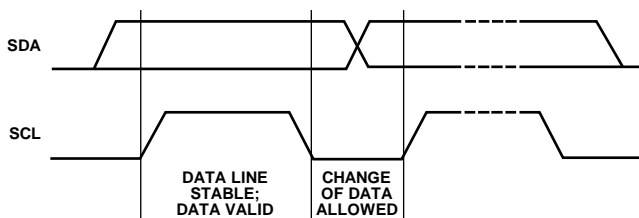
Figure 39. Valid Bit Transfer
