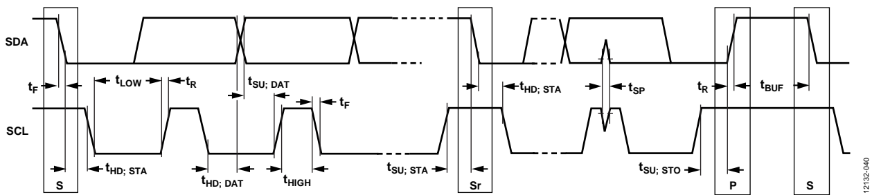
Figure 44. I 2 C Serial Port Timing
