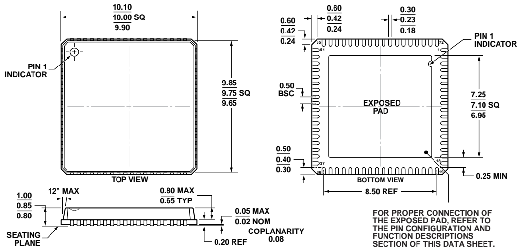
Figure 45. 72-Lead Lead Frame Chip Scale Package [LFCSP_VQ] 10 mm × 10 mm Body, Very Thin Quad (CP-72-4) Dimensions shown in millimeters
