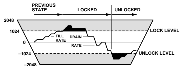
Figure 29. Lock Detector Diagram
