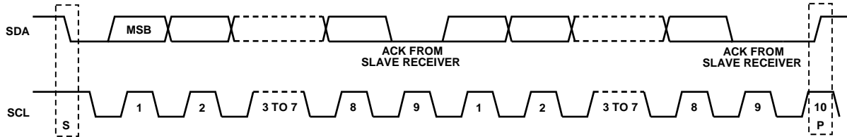
Figure 42. Data Transfer Process (Master Write Mode, 2-Byte Transfer)
