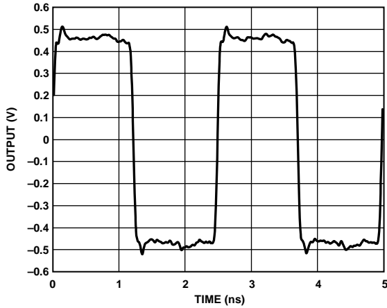
Figure 16. Output Waveform, 14 mA LVDS-Compatible Mode (400 MHz) with 100Ω Termination at Load
