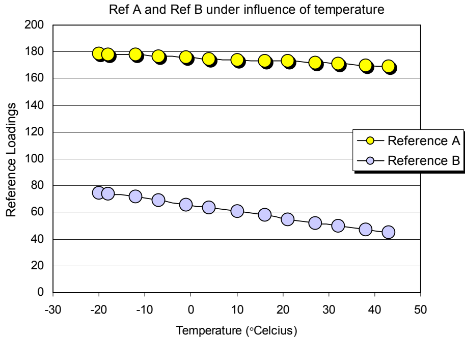
Figure 16. A-to-D Value of Ref A and Ref B Based on Varying Temperature
