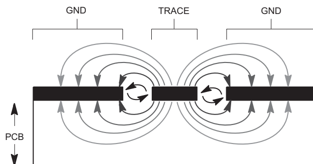
Figure 1. Trace Fringe Capacitance
