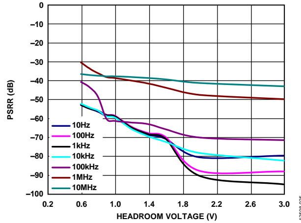
Figure 25. Power Supply Rejection Ratio (PSRR) vs. Headroom Voltage, V_{OUT} = 1.8V , for Different Frequencies
