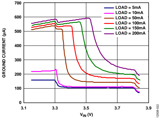
Figure 22. Ground Current vs. Input Voltage ( V_{IN} ) in Dropout, V_{OUT} = 3.3V
