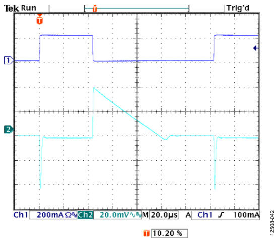
Figure 42. Output Transient Response, V_{OUT} = 5\text{ V} , C_{OUT} = 2.2\ \mu\text{F} , CH1 Load Current, CH2 V_{OUT}
