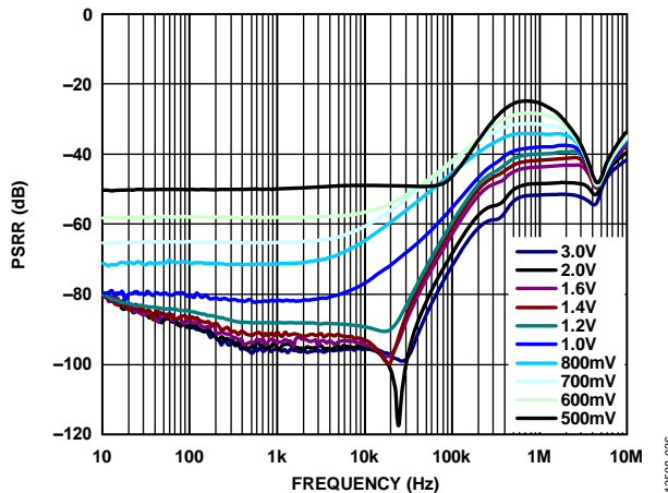
Figure 26. Power Supply Rejection Ratio (PSRR) vs. Frequency, V_{OUT} = 3.3V , for Various Headroom Voltages
