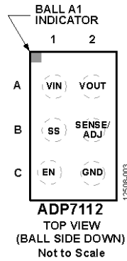
Figure 3. Pin Configuration
