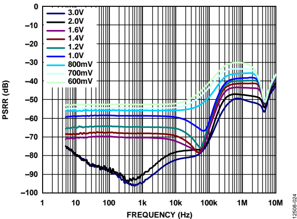
Figure 24. Power Supply Rejection Ratio (PSRR) vs. Frequency, V_{OUT} = 1.8V , for Various Headroom Voltages
