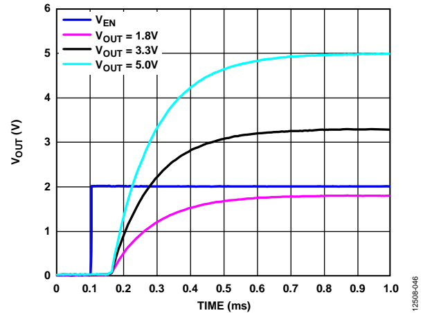
Figure 46. Typical Start-Up Behavior
