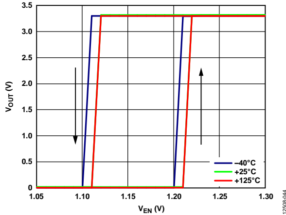
Figure 44. Typical V OUT Response to EN Pin Operation
