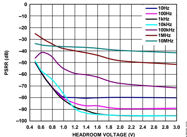
Figure 27. Power Supply Rejection Ratio (PSRR) vs. Headroom Voltage, V_{OUT} = 3.3V , for Different Frequencies
