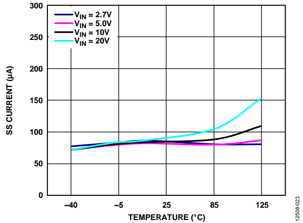
Figure 23. Soft Start (SS) Current vs. Temperature, Multiple Input Voltages, V_{OUT} = 5V
