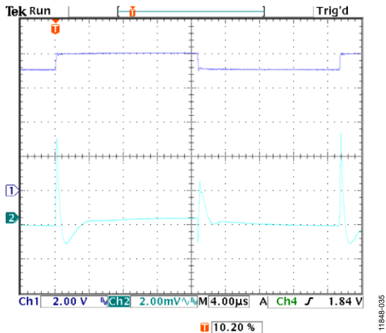
Figure 37. Line Transient Response, I_{LOAD} = 200 \text{ mA} , V_{OUT} = 5 \text{ V} , CH1 V_{IN} , CH2 V_{OUT}
