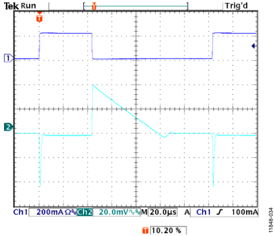
Figure 36. Load Transient Response, I_{LOAD} = 1 \text{ mA to } 200 \text{ mA} , V_{OUT} = 5 \text{ V} , V_{IN} = 7 \text{ V} , CH1 Load Current ( I_{LOAD} ), CH2 V_{OUT}
