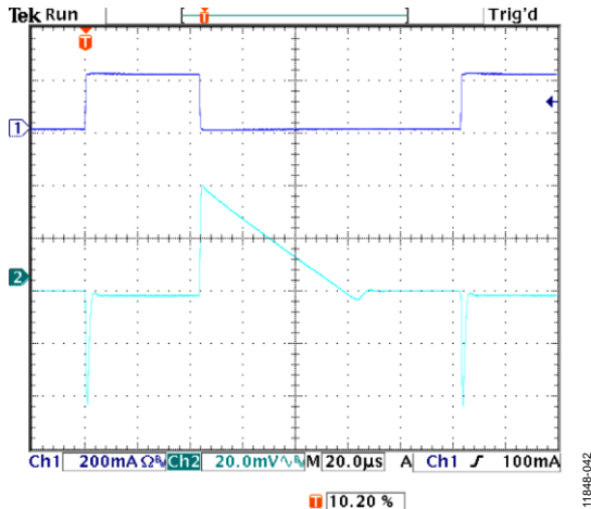
Figure 44. Output Transient Response, V_{\text{OUT}} = 5\text{ V} , C_{\text{OUT}} = 2.2\ \mu\text{F} , CH1 Load Current, CH2 V_{\text{OUT}}
