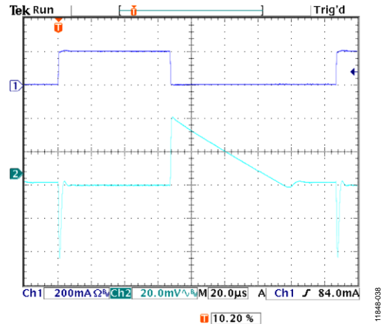
Figure 40. Load Transient Response, I_{LOAD} = 1 \text{ mA to } 200 \text{ mA} , V_{OUT} = 1.8 \text{ V} , V_{IN} = 3 \text{ V} , CH1 Load Current ( I_{LOAD} ), CH2 V_{OUT}
