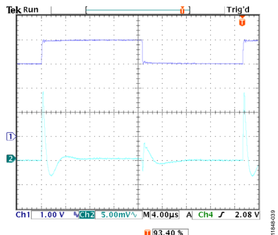
Figure 41. Line Transient Response, I_{LOAD} = 200 \text{ mA} , V_{OUT} = 1.8 \text{ V} , CH1 V_{IN} , CH2 V_{OUT}
