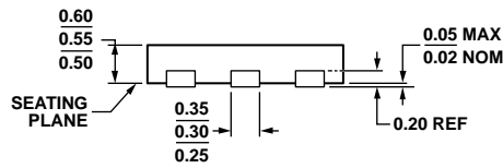
Figure 67. 6-Lead Lead Frame Chip Scale Package [LFCSP_UD] 2.00 mm x 2.00 mm Body, Ultra Thin, Dual Lead (CP-6-3) Dimensions shown in millimeters
