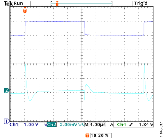
Figure 39. Line Transient Response, I_{LOAD} = 200 \text{ mA} , V_{OUT} = 3.3 \text{ V} , CH1 V_{IN} , CH2 V_{OUT}
