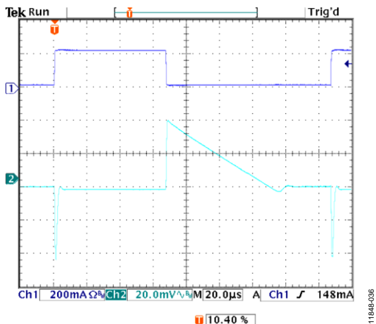
Figure 38. Load Transient Response, I_{LOAD} = 1 \text{ mA to } 200 \text{ mA} , V_{OUT} = 3.3 \text{ V} , V_{IN} = 5 \text{ V} , CH1 Load Current ( I_{LOAD} ), CH2 V_{OUT}
