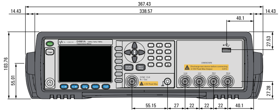
Figure 14. Dimensions (front view, with handle and bumper, in millimeters, nominal)
