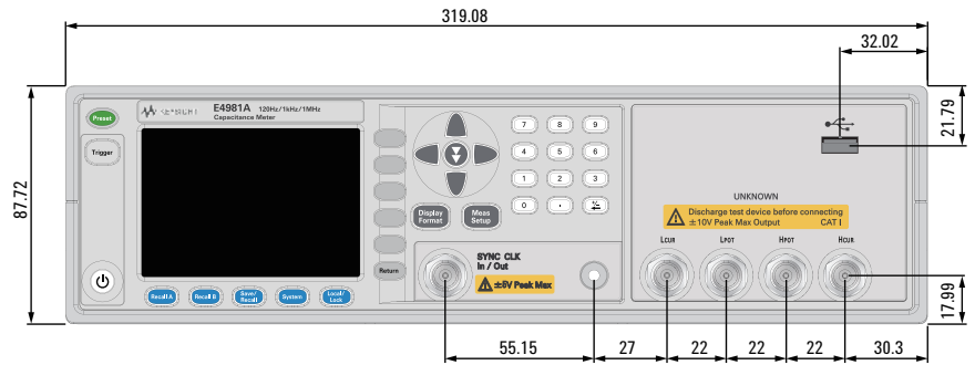
Figure 15. Dimensions (front view, without handle and bumper, in millimeters, nominal)
