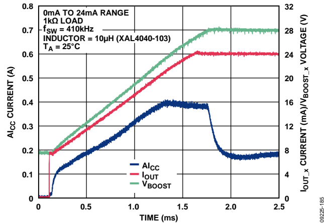
Figure 60. I_{CC} Current vs. Time for 24 mA Step Through 1 k \Omega Load with External 51 k \Omega Compensation Resistor
