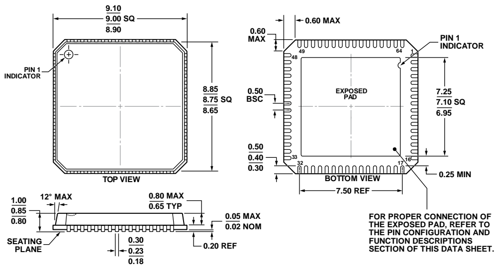
COMPLIANT TO JEDEC STANDARDS MO-220-VMM4-4 Figure 68. 64-Lead Lead Frame Chip Scale Package [LFCSP_VQ] 9 mm × 9 mm Body, Very Thin Quad (CP-64-3) Dimensions shown in millimeters
