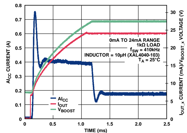
Figure 59. AI_{CC} Current vs. Time for 24 mA Step Through 1 k \Omega Load with Internal Compensation Resistor
