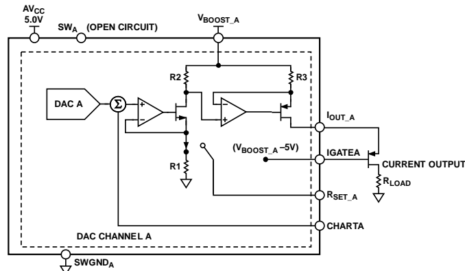
Figure 63. Configuration of a Particular Channel Using IGATE
