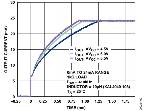
Figure 29. Output Current Settling with DC-to-DC Converter vs. Time and V_{CC} (See Figure 57)
