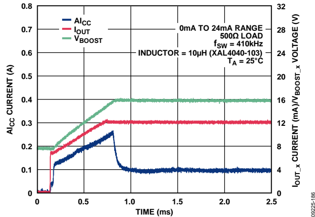
Figure 61. I_{CC} Current vs. Time for 24 mA Step Through 500 \Omega Load with External 51 k \Omega Compensation Resistor
