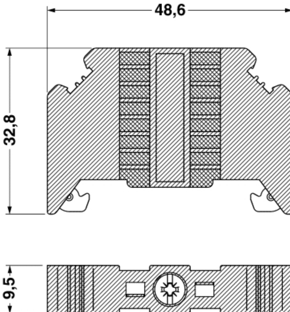
Dimensioned drawing
