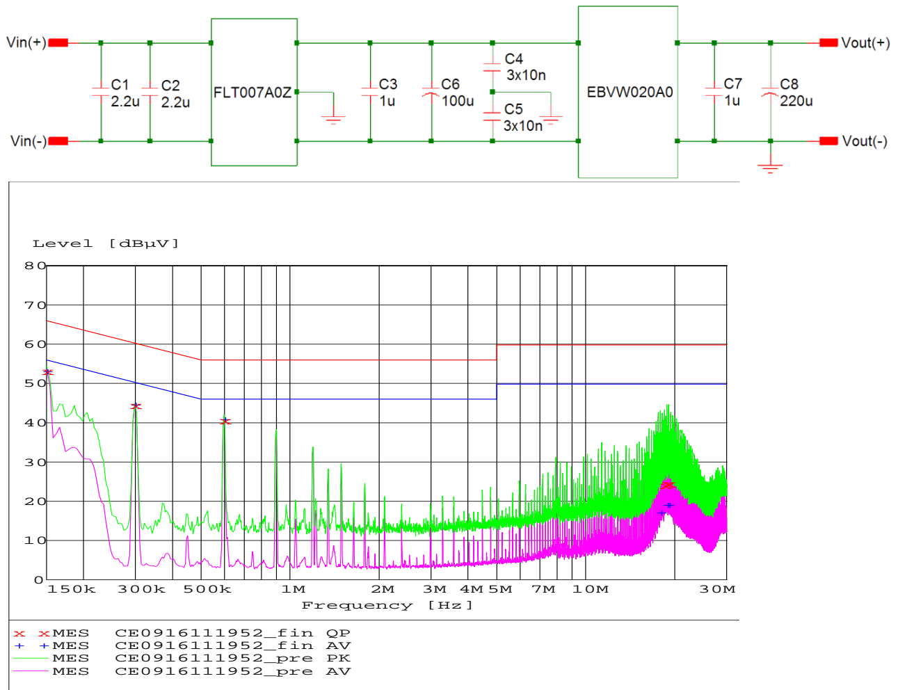
Figure 24. EMC Considerations.
