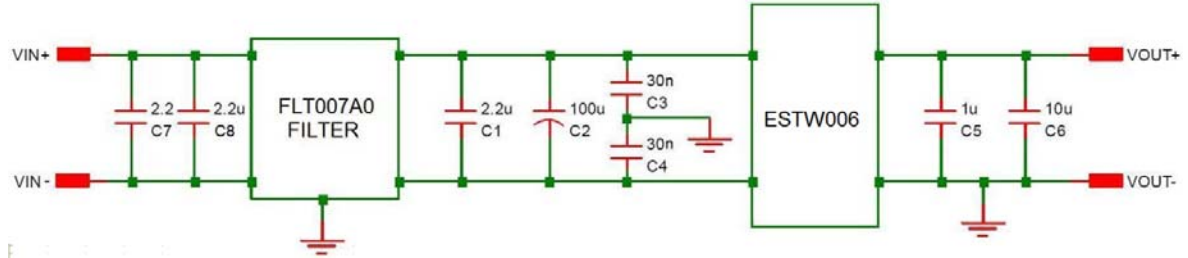
Figure 26. EMC Considerations.
