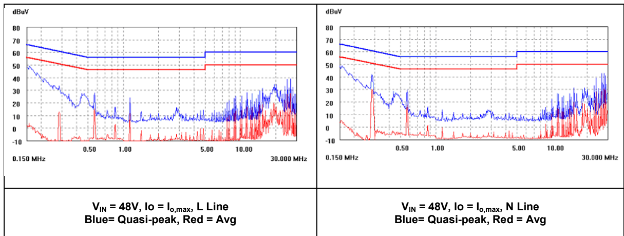
Figure 26. EMC Considerations.
