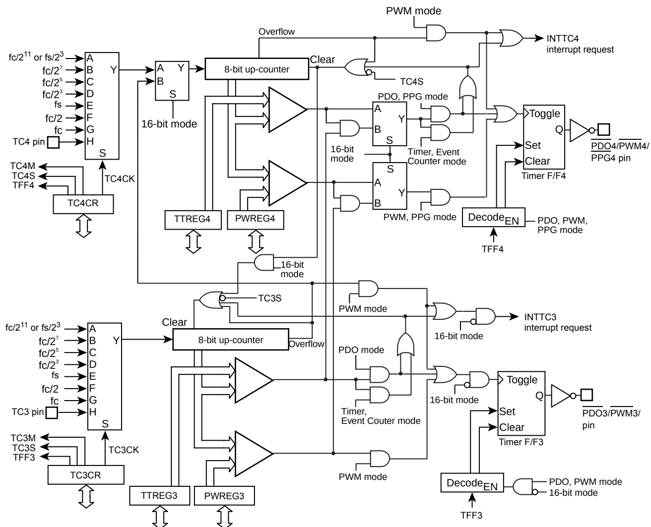
Figure 10-1 8-Bit TimerCounter 3, 4
