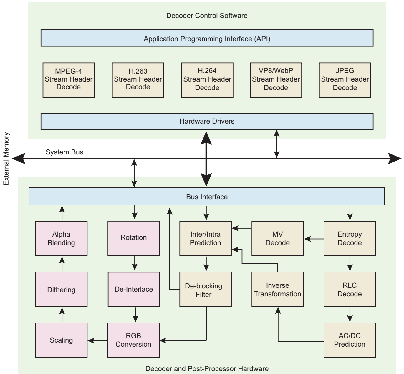
Figure 33-1. Block Diagram
