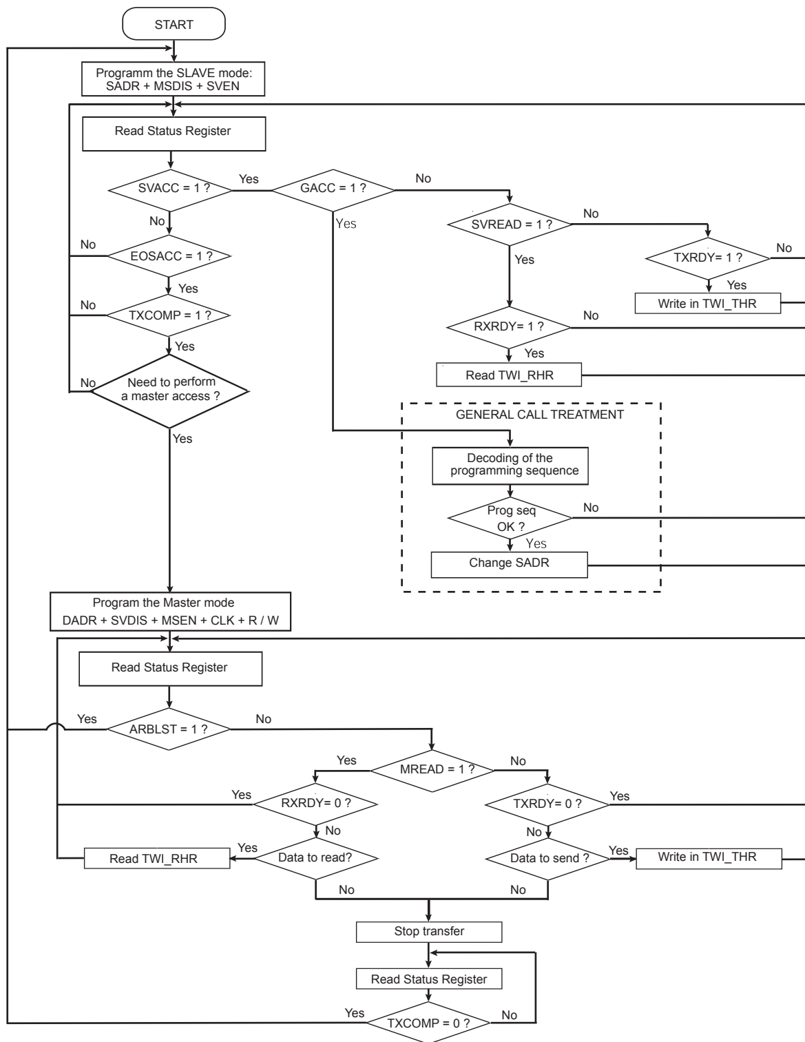
Figure 40-23. Multi-master Flowchart
