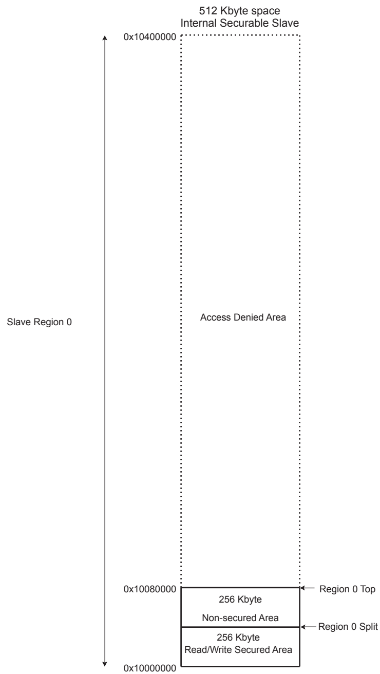
Figure 16-2. Partitioning example of an Internal Securable slave featuring 1 security region of 512 KB split into 1 or 2 security areas of 4 KB to 512 KB
