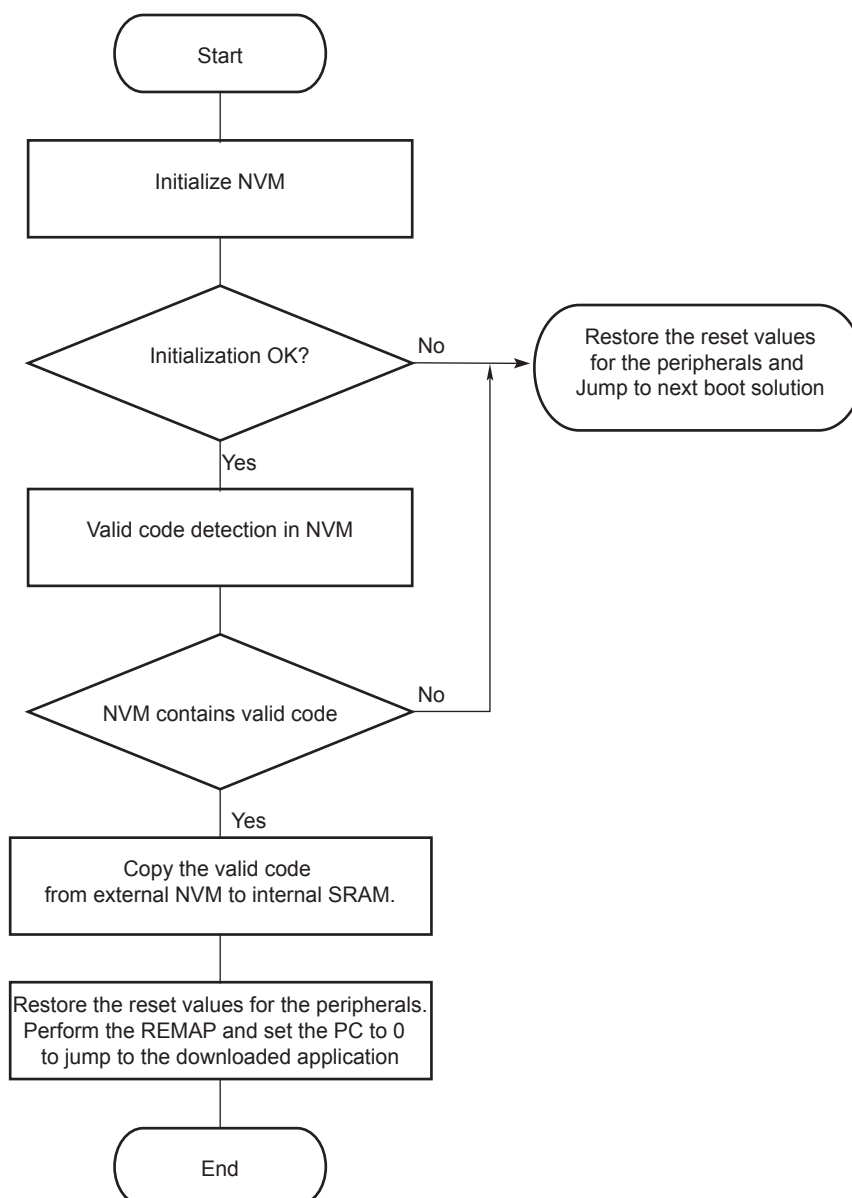
Figure 13-3. NVM Bootloader Program Diagram
