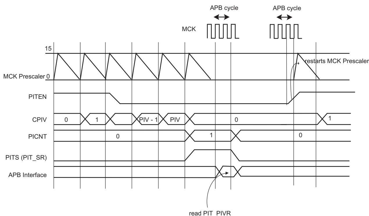
Figure 22-2. Enabling/Disabling PIT with PITEN
