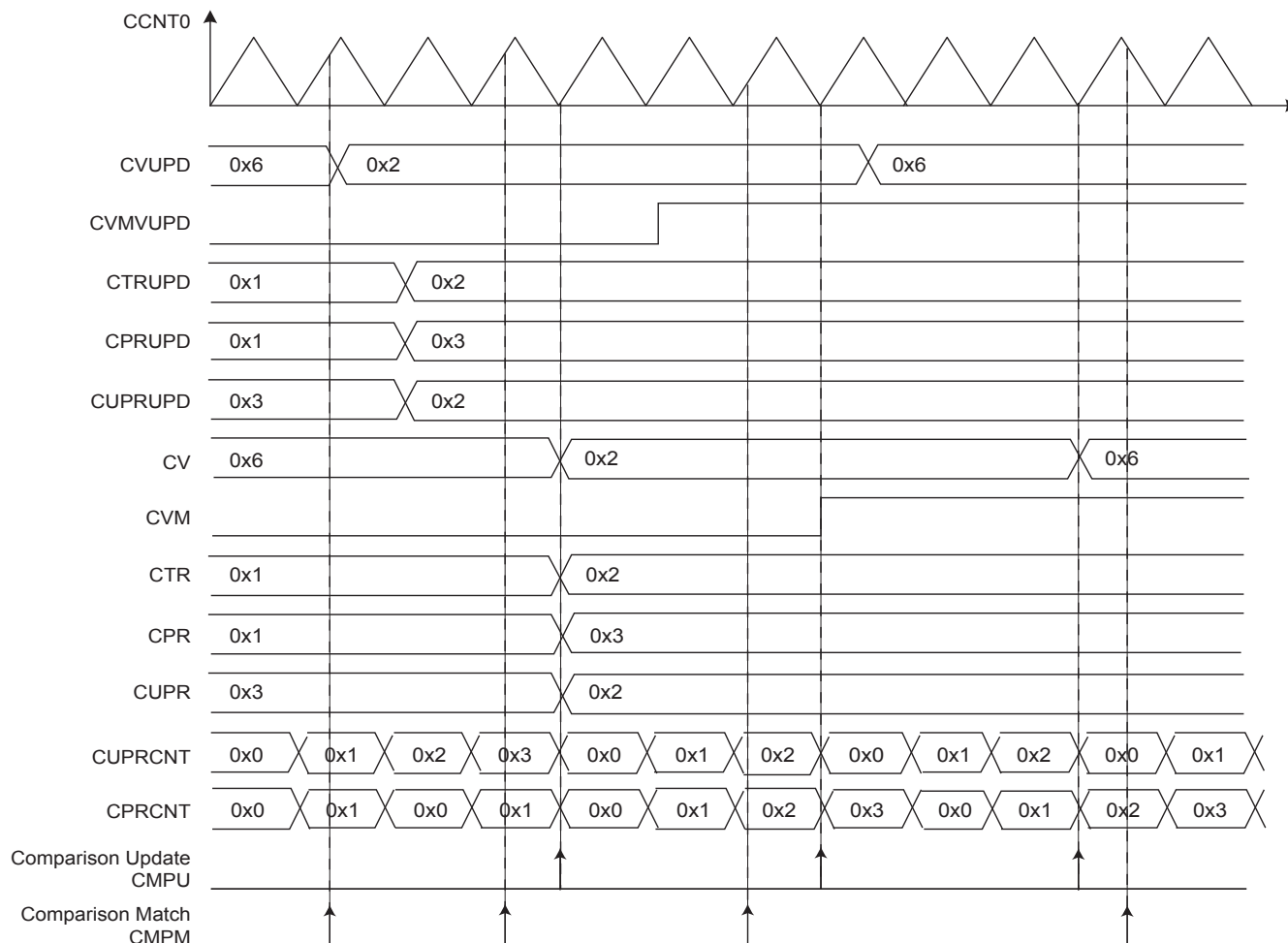
Figure 47-16. Comparison Waveform
