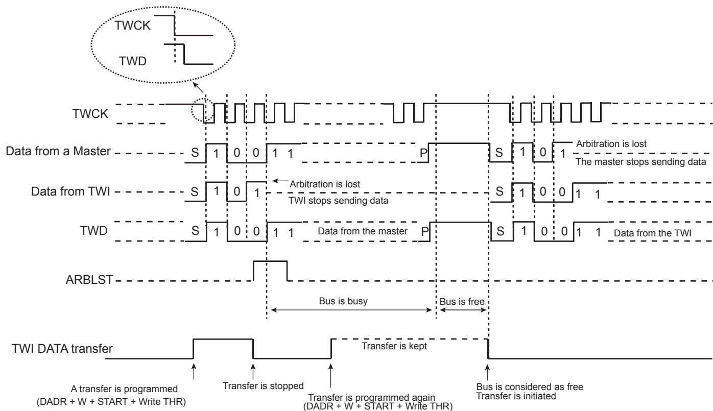
Figure 40-22. Arbitration Cases
