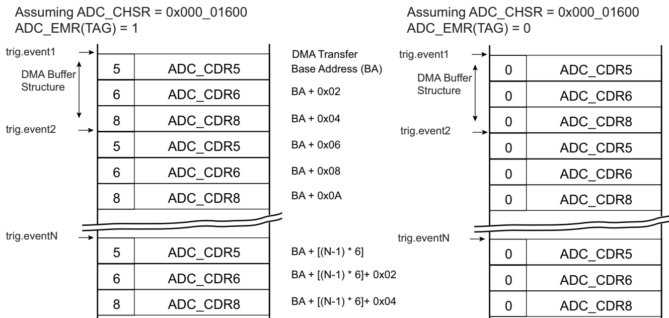
Figure 48-16. Buffer Structure
