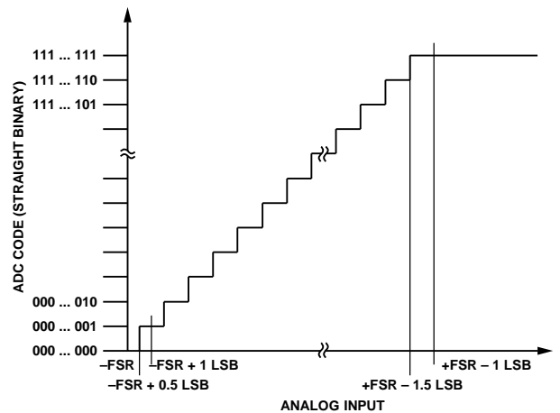
Figure 32. ADC Ideal Transfer Function
