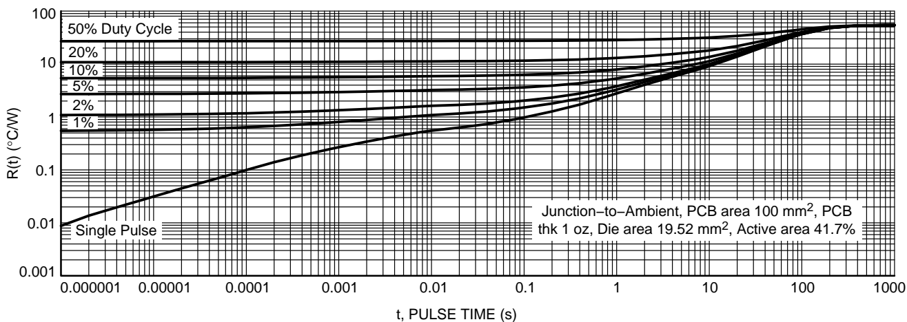
Figure 9. Thermal Characteristics
