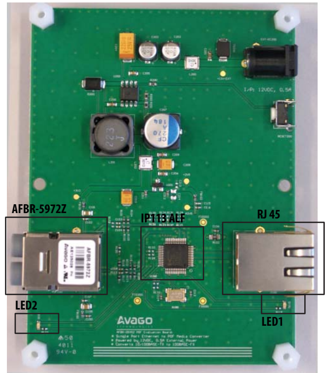
Figure 3. AFBR-0545Z media converter evaluation board
