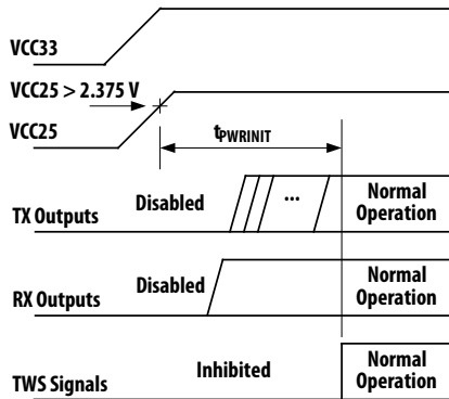
Figure 18. Power-up Sequence
