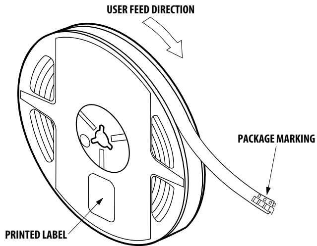
Figure 14. Reeling orientation
