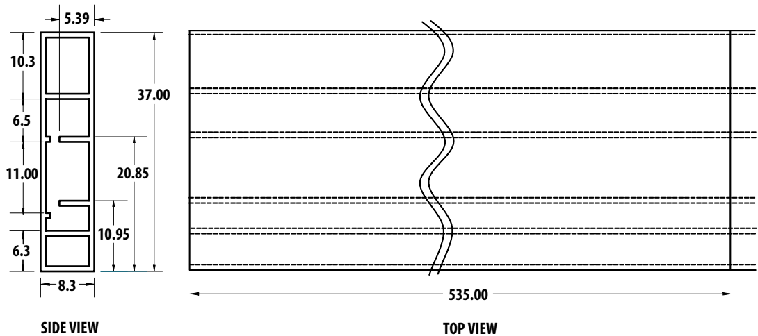
Figure 17. Tube dimensions.
