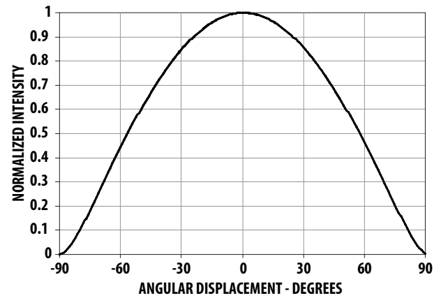
Figure 7. Radiation Pattern.
