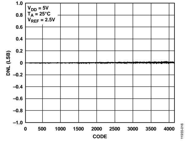
Figure 16. AD5681R DNL
