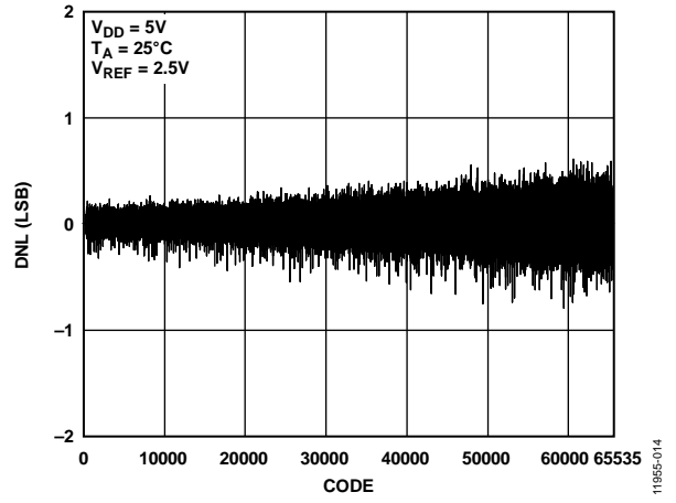
Figure 14. AD5683R/AD5683 DNL
