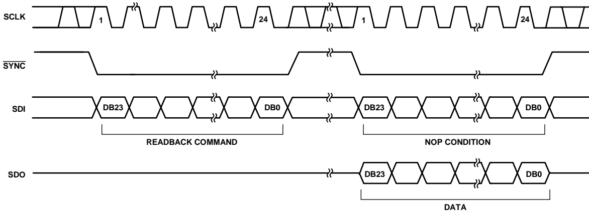
Figure 53. Readback Operation
