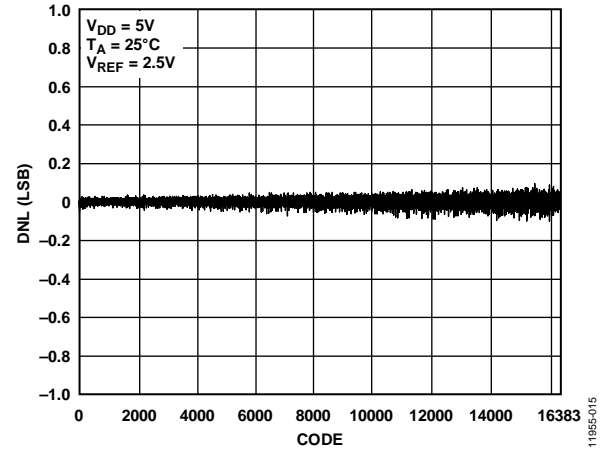
Figure 15. AD5682R DNL
