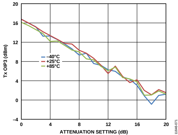
Figure 71. Tx Third-Order Output Intercept Point (OIP3) vs. Attenuation Setting, f_{LO\_TX} = 5.8 GHz
