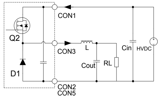
Buck
