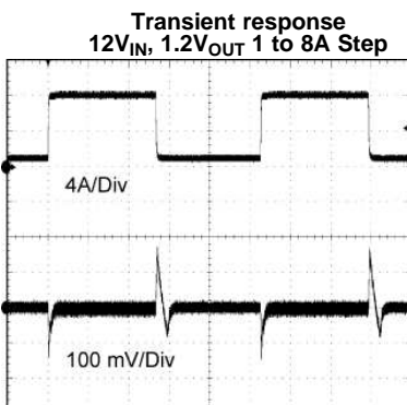
TIME (500 \mu s/Div) Figure 46.
