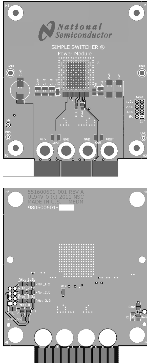
Figure 56. Layout Example
