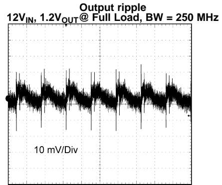
TIME (2 \mu s/Div) Figure 43.
