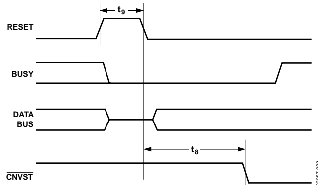
Figure 24. Reset Timing
