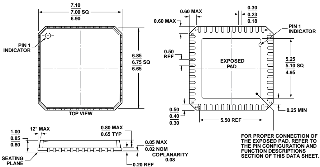
Figure 37. 48-Lead Lead Frame Chip Scale Package [LFCSP_VQ] 7 mm x 7 mm Body, Thin Quad (CP-48-1)
