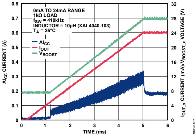
Figure 61. A_{lcc} Current vs. Time for 24 mA Step Through 1 kΩ Load with Slew Rate Control
