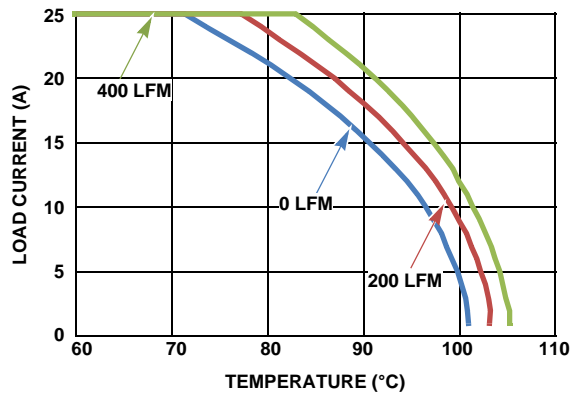
FIGURE 19. 12V_{IN} TO 1.8V_{OUT}
