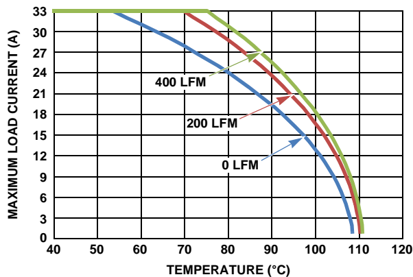
FIGURE 19. 5V_{IN} TO 1.8V_{OUT}
