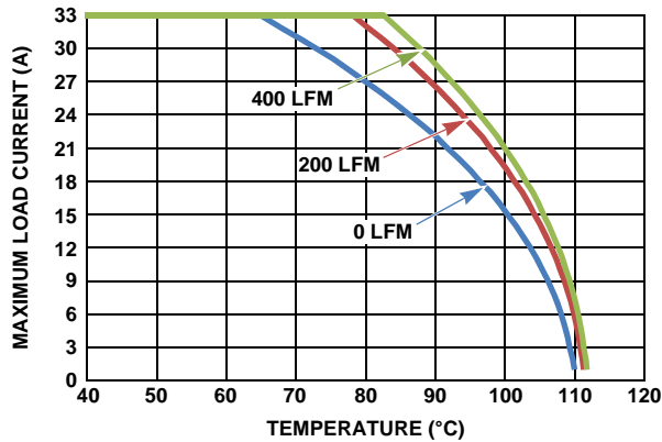
FIGURE 15. 5V_{IN} TO 1V_{OUT}
