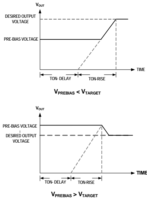
FIGURE 27. OUTPUT RESPONSES TO PRE-BIAS VOLTAGES
