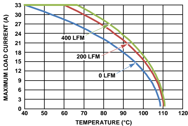
FIGURE 23. 5V_{IN} TO 3.3V_{OUT}
