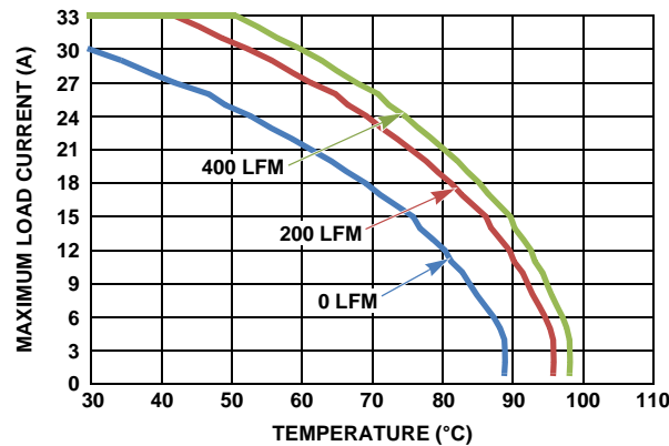
FIGURE 25. 12V_{IN} TO 5V_{OUT} , 700kHz
