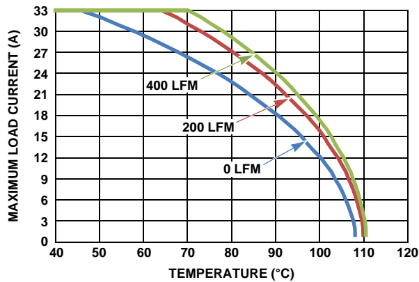
FIGURE 21. 5V_{IN} TO 2.5V_{OUT}
