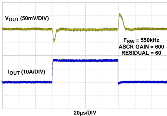
FIGURE 9. LOAD TRANSIENT RESPONSE AT V_{IN} = 12\text{V} , V_{OUT} = 1\text{V} WITH HIGH BANDWIDTH ASCR PARAMETER
