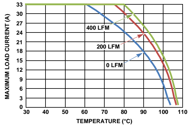
FIGURE 16. 12V_{IN} TO 1V_{OUT}
