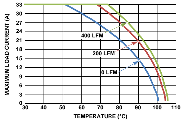
FIGURE 20. 12V_{IN} TO 1.8V_{OUT}
