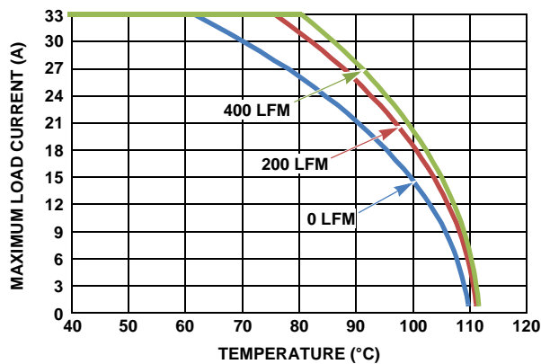
FIGURE 17. 5V_{IN} TO 1.2V_{OUT}
