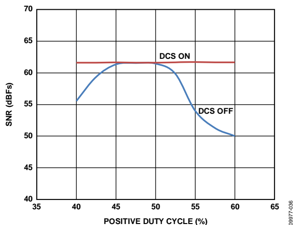
Figure 58. SNR vs. DCS On/Off
