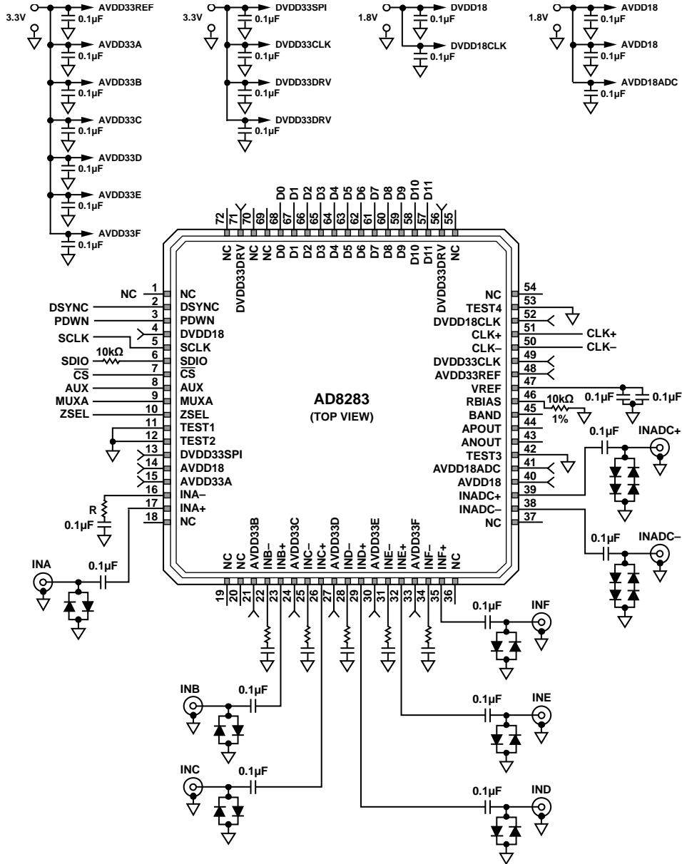
Figure 34. Single-Ended Inputs
