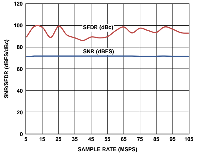
Figure 32. SNR/SFDR vs. Sample Rate with AIN = 70.1 MHz
