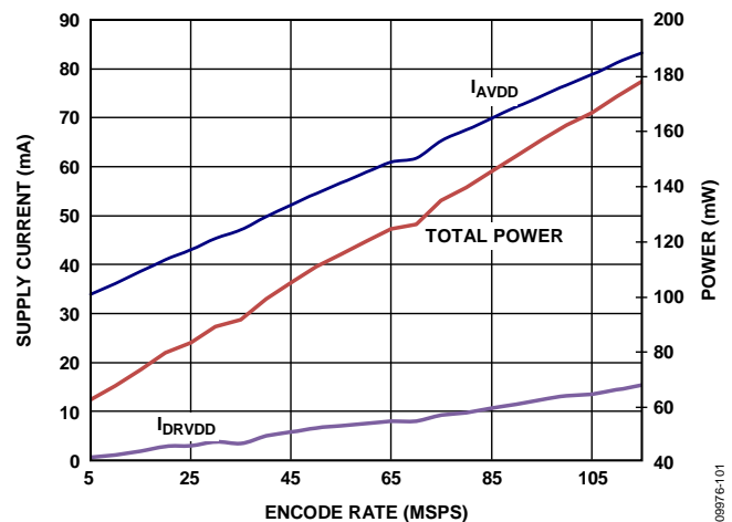
Figure 61. AD9628-105 Power and Current vs. Clock Rate (1.8 V CMOS Output Mode)
