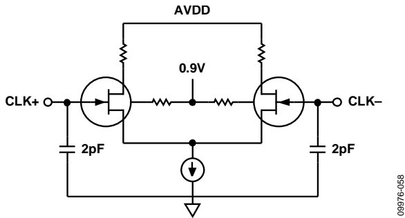
Figure 52. Equivalent Clock Input Circuit
