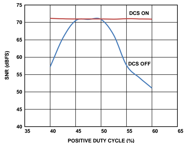
Figure 58. SNR vs. DCS On/Off
