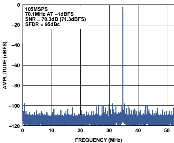
Figure 25. Single-Tone FFT with f_{IN} = 70.1 MHz
