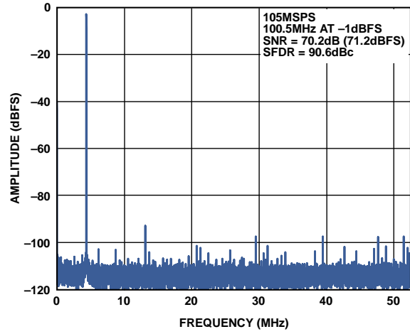
Figure 26. Single-Tone FFT with f_{IN} = 100.5 MHz
