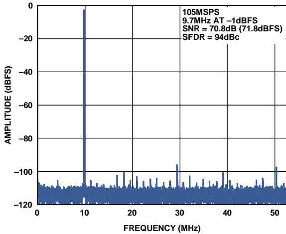
Figure 23. Single-Tone FFT with f_{IN} = 9.7 MHz
