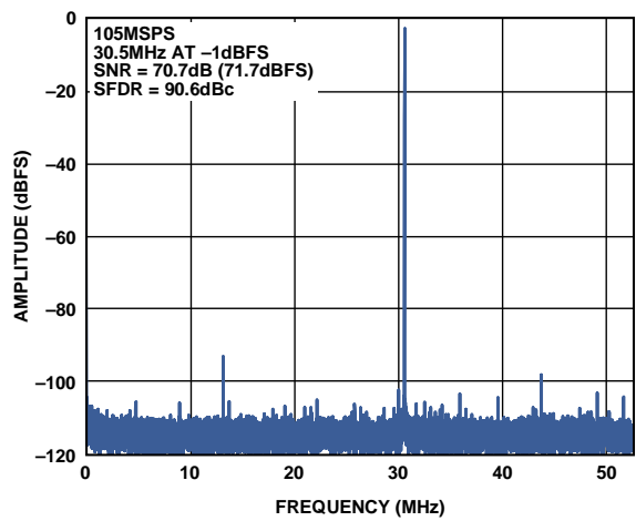
Figure 24. Single-Tone FFT with f_{IN} = 30.5 MHz
