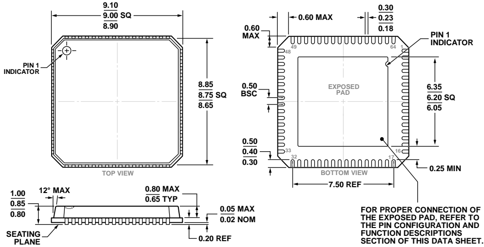
Figure 63. 64-Lead Lead Frame Chip Scale Package [LFCSP_VQ] 9 mm × 9 mm Body, Very Thin Quad (CP-64-4) Dimensions shown in millimeters
