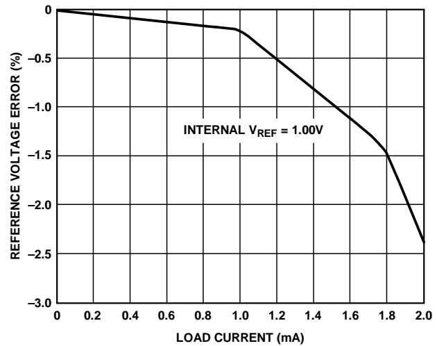
Figure 50. VREF Accuracy vs. Load Current
