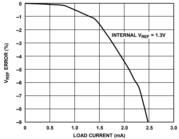
Figure 59. V_{REF} = 1.3\text{ V} Error vs. Load Current
