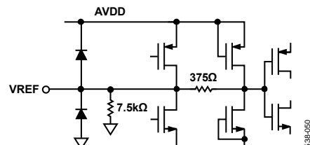
Figure 50. Equivalent VREF Circuit
