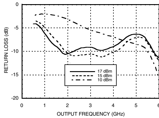
Output Return Loss with 2.5 GHz Input
