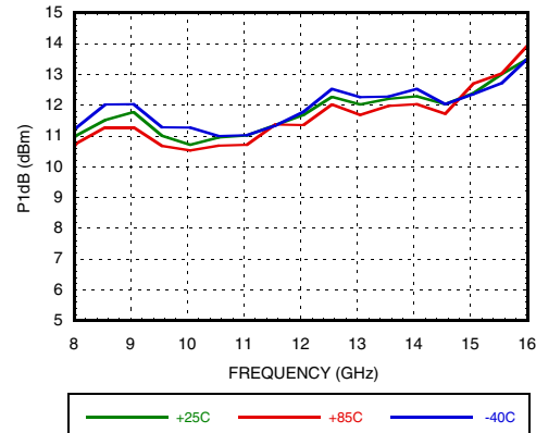
Input P1dB vs. Temperature @ LO = +13 dBm
