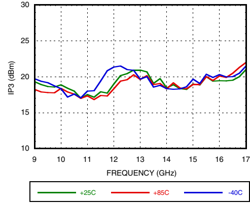
Input IP3 vs. Temperature @ LO = +13 dBm [1]
