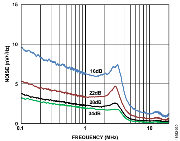
Figure 12. Short-Circuit Input Referred Noise vs. Frequency
