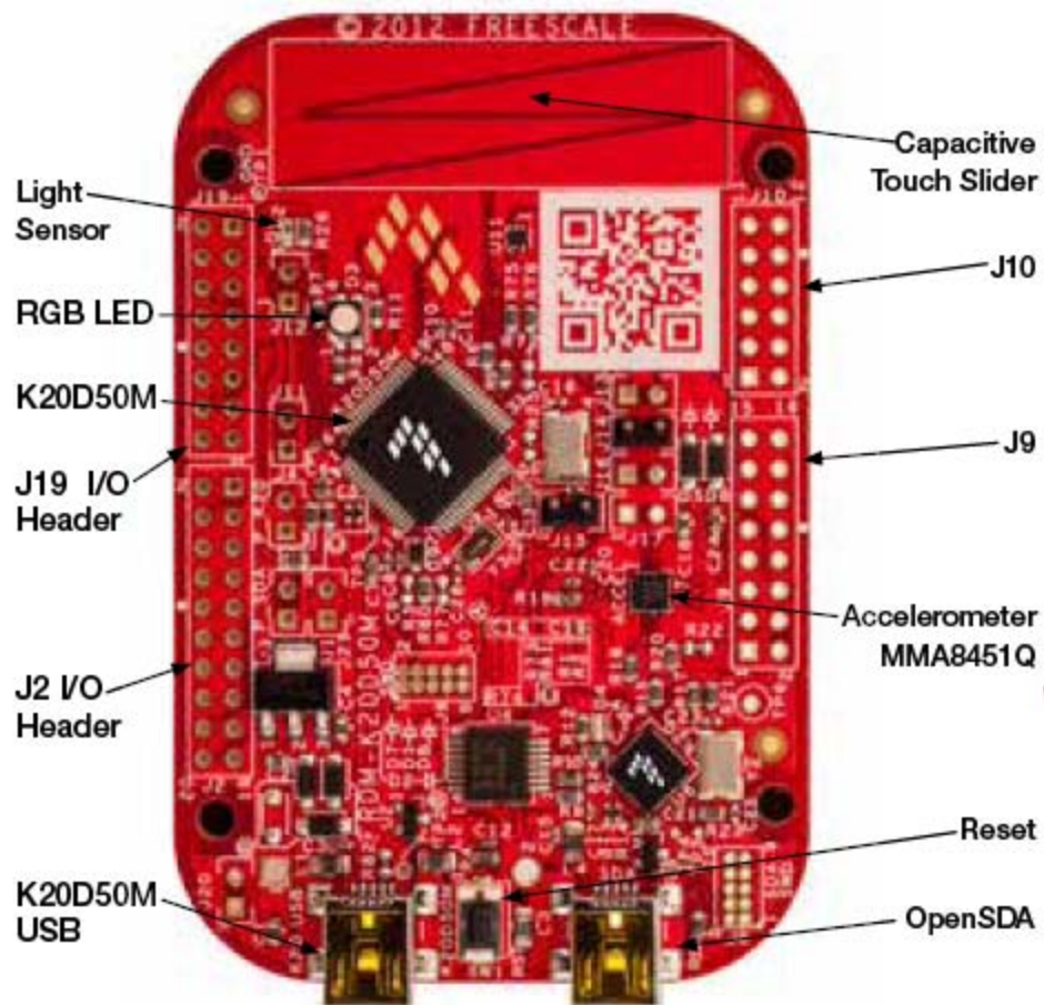
Figure 1: FRDM-K20D50M Callouts
