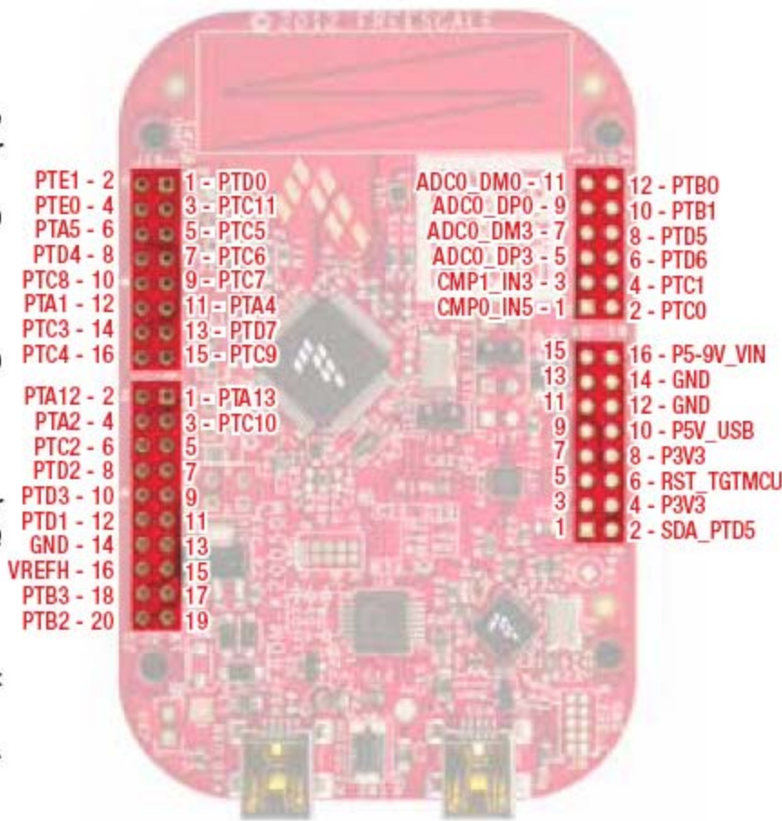
Figure 2: FRDM-K20D50M Pin-Out
