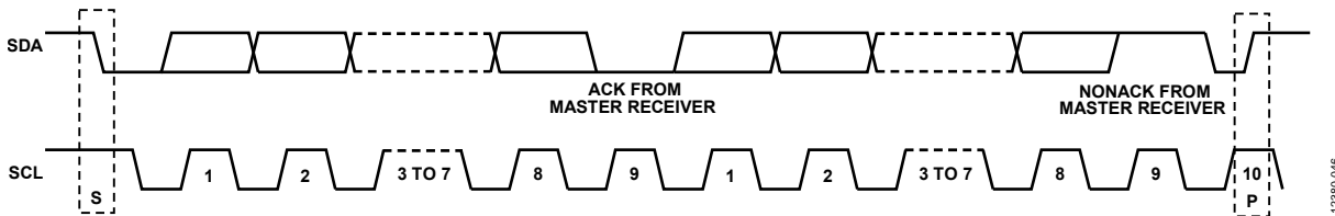
Figure 49. Data Transfer Process (Master Read Mode, 2-Byte Transfer), First ACK From Slave
