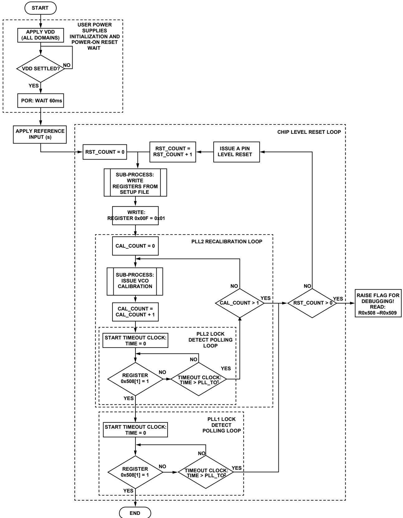
Figure 51. Main Process, Initialization
