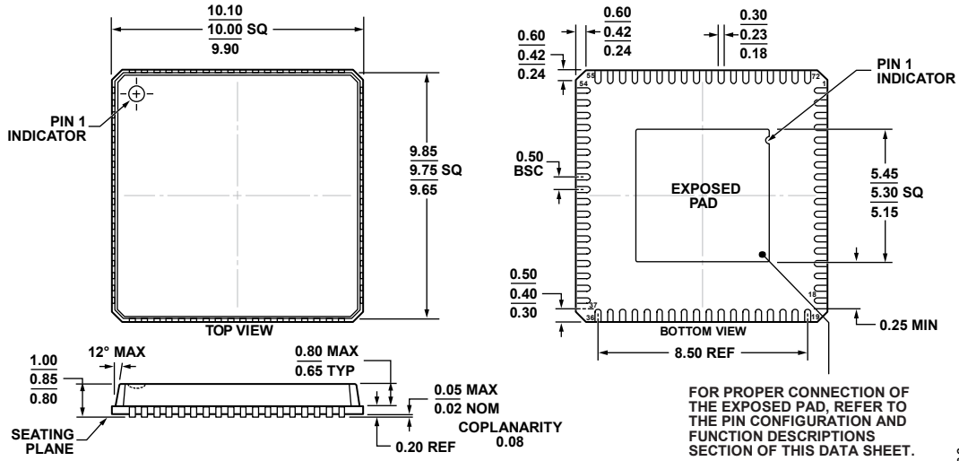
Figure 55. 72-Lead Lead Frame Chip Scale Package [LFCSP_VQ] 10 mm × 10 mm Body, Very Thin Quad (CP-72-6) Dimensions shown in millimeters
