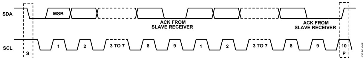
Figure 48. Data Transfer Process (Master Write Mode, 2-Byte Transfer)
