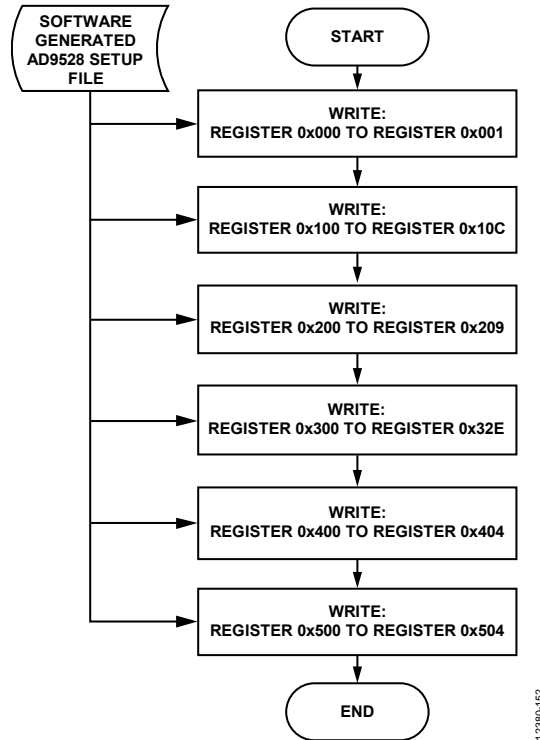
Figure 54. Subprocess, Write Registers from the Setup File
