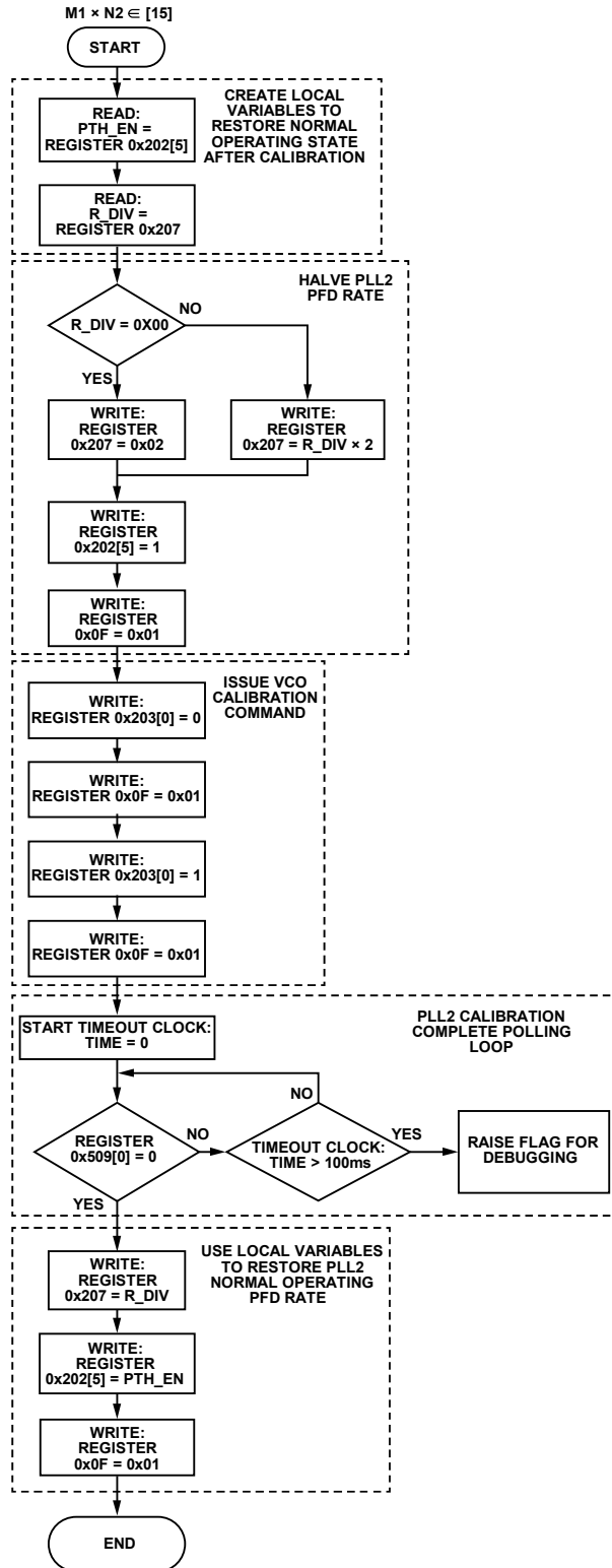
Figure 53. Subprocess, Issue VCO Calibration ( M1 \times N2 = 15 )
