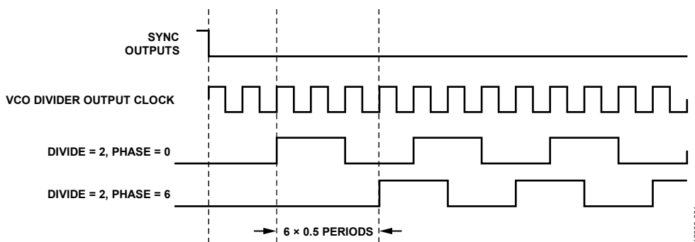
Figure 35. Clock Output Synchronization Timing Diagram
