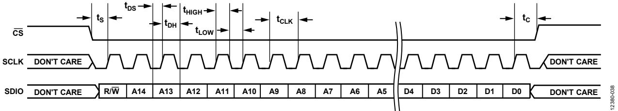
Figure 41. Timing Diagram for Serial Control Port Write—MSB First
