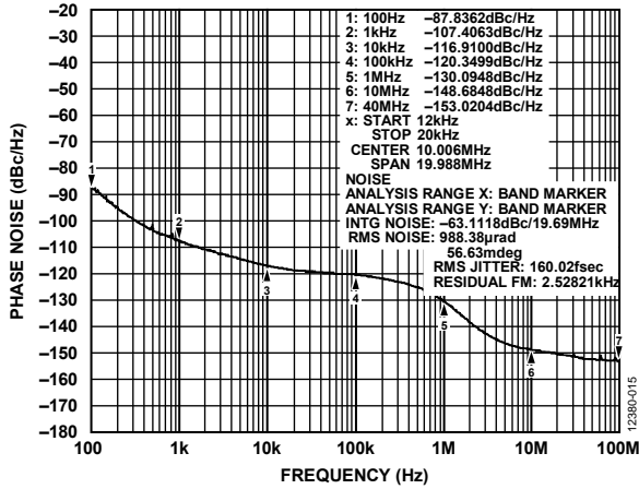
Figure 15. Phase Noise, Output = 983.04 MHz, Dual Loop Mode (VCXO = 122.88 MHz, Crystek VCXO CVHD-950, VCO = 3932.16 MHz)
