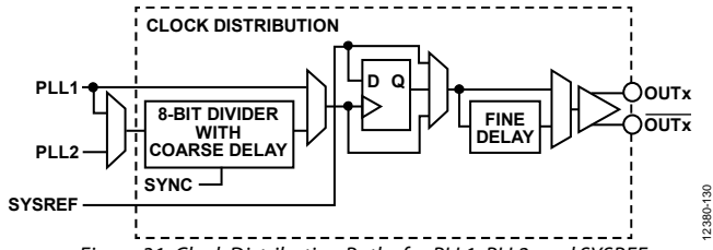
Figure 31. Clock Distribution Paths for PLL1, PLL2, and SYSREF Frequency Sources
