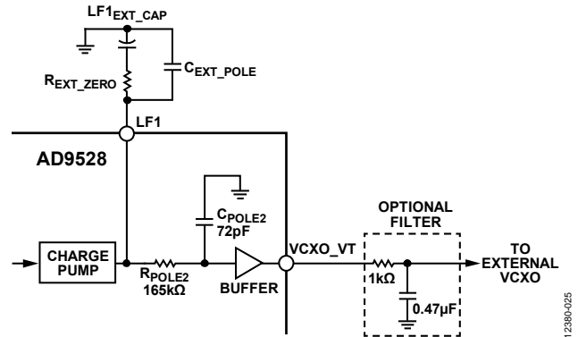
Figure 27. PLL1 Loop Filter
