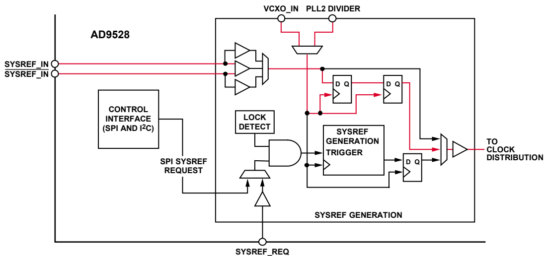
Figure 37. Mode 2, Retimes the External SYSREF to the Internal VCXO or PLL2 Input Divider Output and then Routes to the Clock Distribution Output(s)
