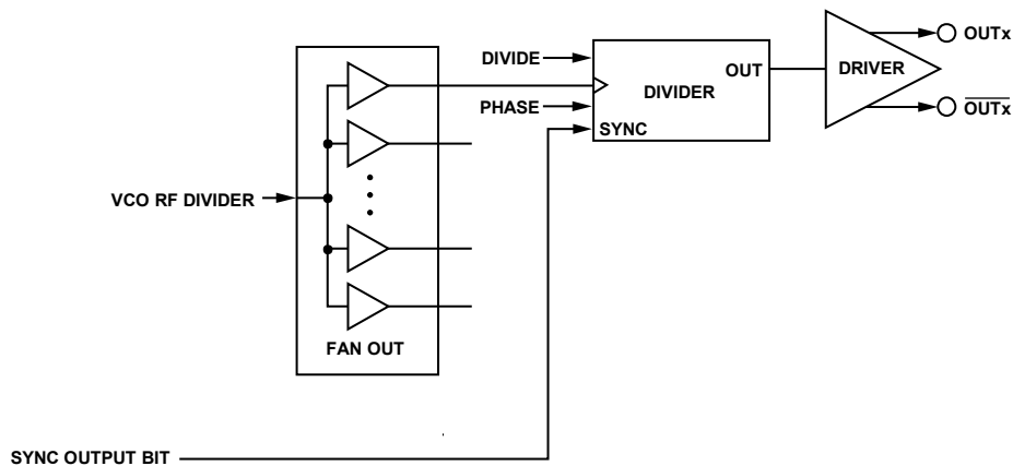
Figure 34. Clock Distribution Synchronization Block Diagram
