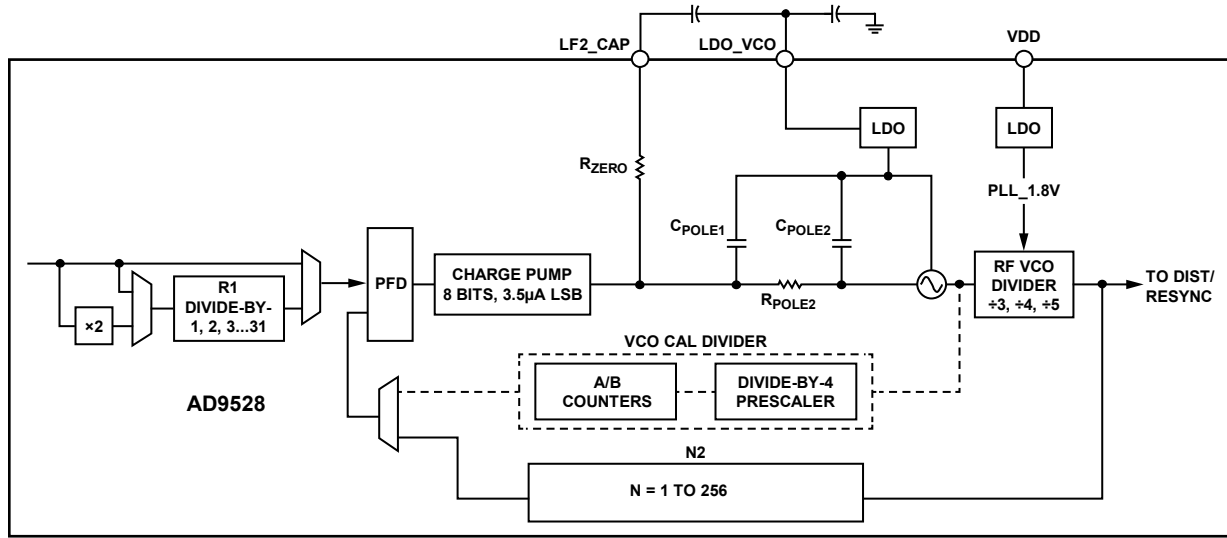
Figure 29. PLL2 Block Diagram
