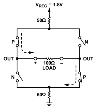
Figure 33. HSTL Output Driver
