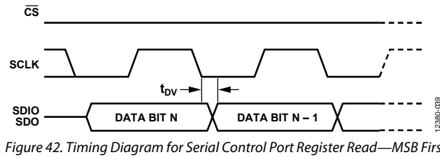
Figure 42. Timing Diagram for Serial Control Port Register Read—MSB First
