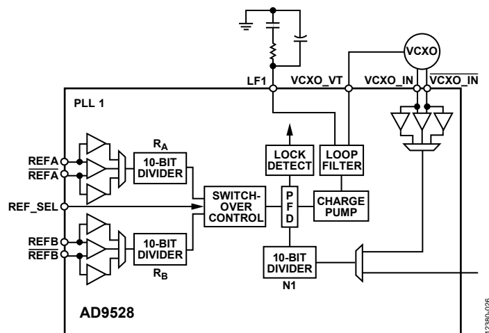
Figure 28. Input PLL (PLL1) Block Diagram
