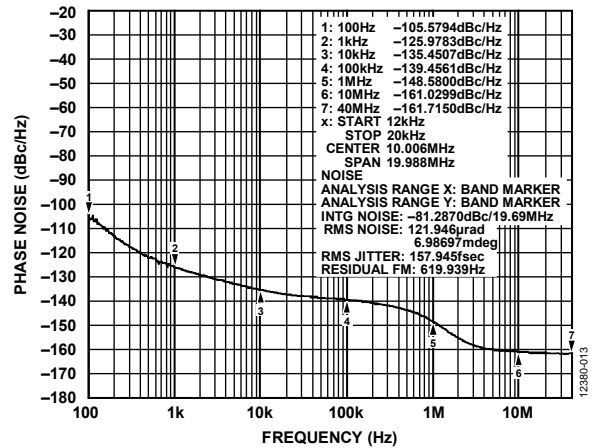
Figure 13. Phase Noise, Output = 122.88 MHz, Dual Loop Mode (VCXO = 122.88 MHz, Crystek VCXO CVHD-950, VCO = 3686.4 MHz)
