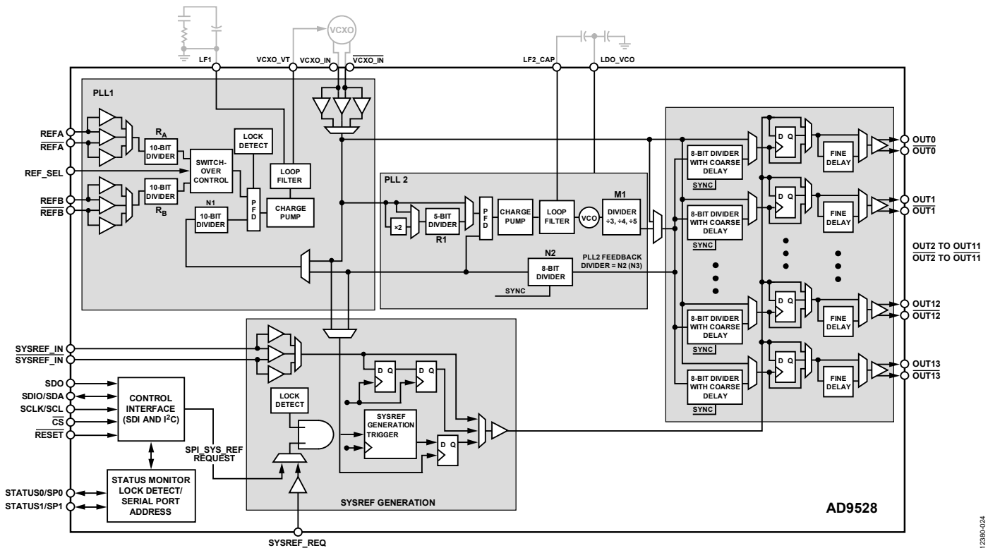
Figure 26. Top Level Diagram
