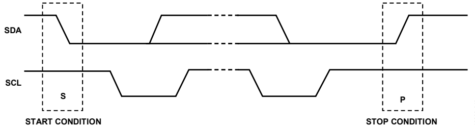
Figure 46. Start and Stop Conditions
