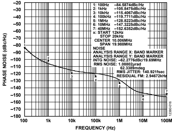
Figure 16. Phase Noise, Output = 1228.8 MHz, Dual Loop Mode (VCXO = 122.88 MHz, Crystek VCXO CVHD-950, VCO = 3686.4 MHz)
