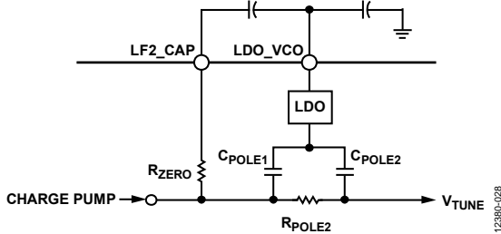
Figure 30. PLL2 Loop Filter
