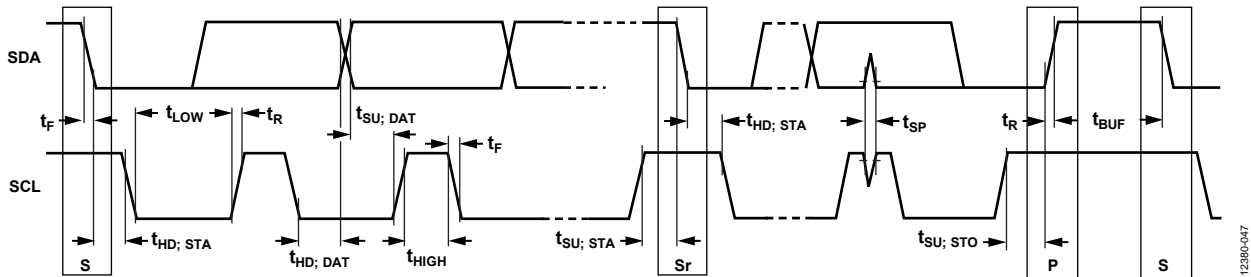
Figure 50. I 2 C Serial Port Timing
