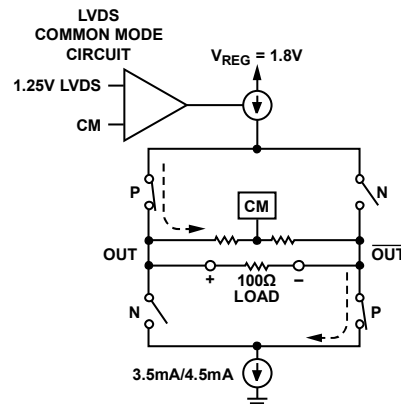
Figure 32. LVDS Output Driver
