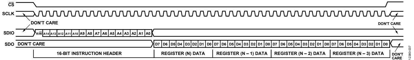
Figure 40. Serial Control Port Read—MSB First, Address Decrement, Four Bytes of Data
