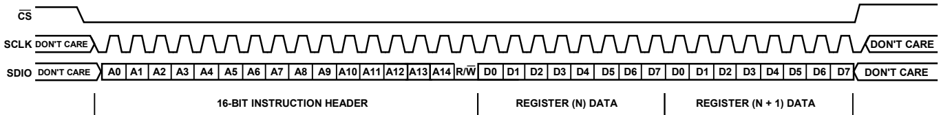
Figure 43. Serial Control Port Write—LSB First, Address Increment, Two Bytes of Data
