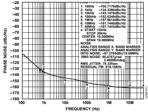
Figure 17. Phase Noise, Output = 122.88 MHz, PLL1 Output Sent Directly to Clock Distribution, PLL2 Off (VCXO = 122.88 MHz, TAITEN VCXO (A0145-0-011-3))
