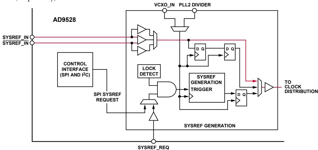
Figure 36. Mode 1, Routes the External SYSREF Directly to the Clock Distribution Output(s)
