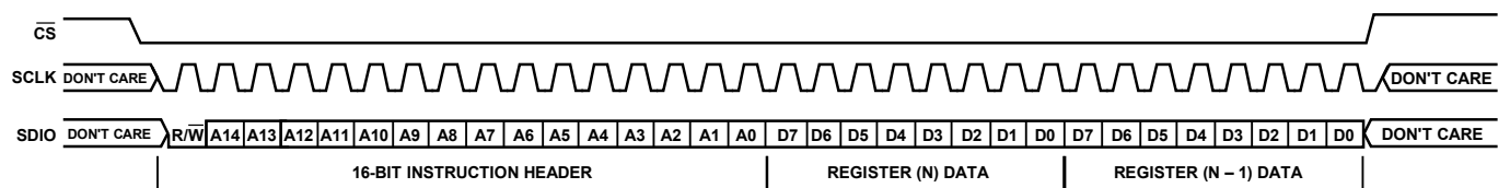
Figure 39. Serial Control Port Write—MSB First, Address Decrement, Two Bytes of Data
