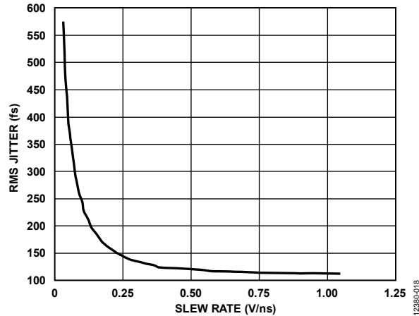
Figure 18. RMS Jitter in Buffer Mode with Both PLL1 and PLL2 Off vs. Slew Rate; Input Applied to the VCXO Input and Output Taken from Clock Distribution, Phase Noise Integration Range from 12 kHz to 20 MHz to Derive Jitter Number
