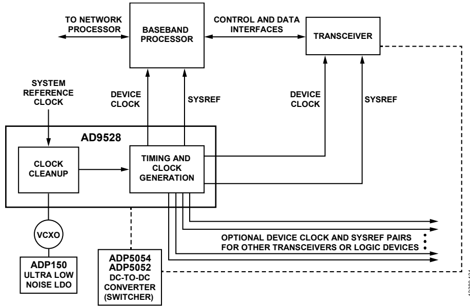
Figure 25. Synchronizing Multiple JESD204B Devices
