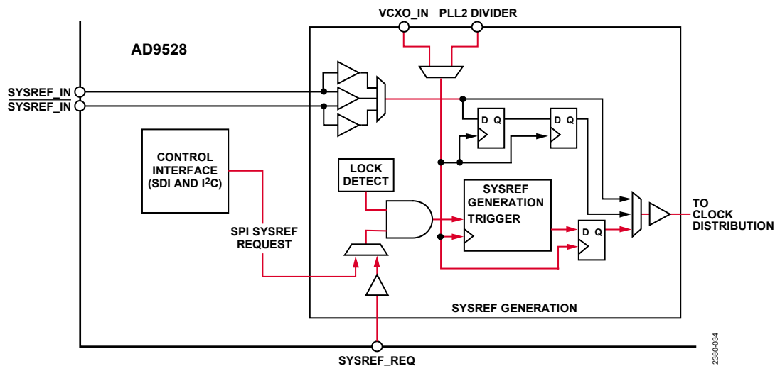
Figure 38. Mode 3, SYSREF Generated Internally and Routed to the Clock Distribution
