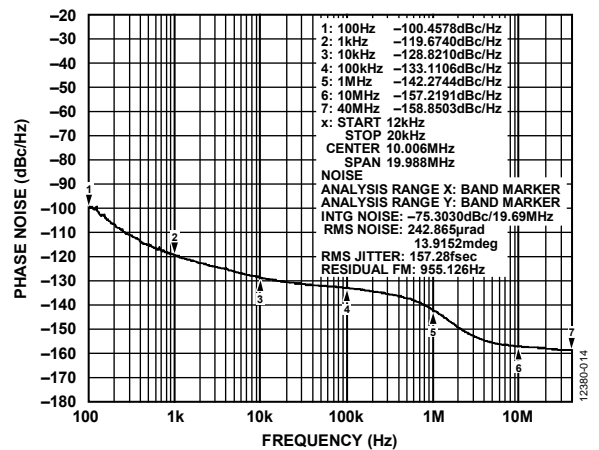
Figure 14. Phase Noise, Output = 245.76 MHz (VCXO = 122.88 MHz, Crystek VCXO CVHD-950, VCO = 3686.4 MHz)
