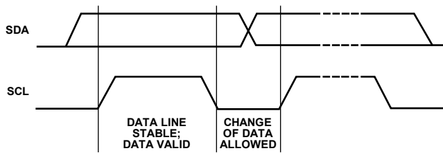
Figure 45. Valid Bit Transfer
