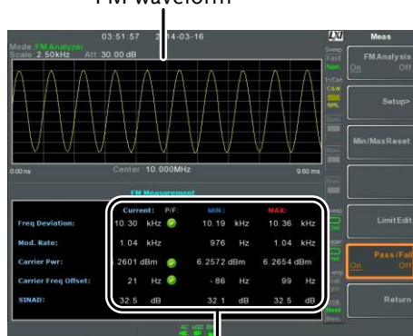
FM modulation measurements
