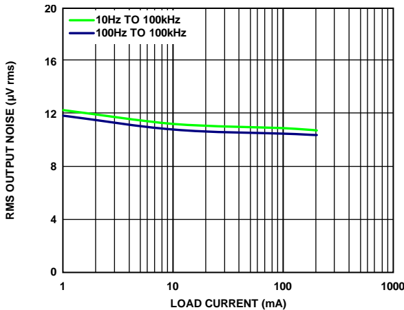
Figure 30. RMS Output Noise vs. Load Current
