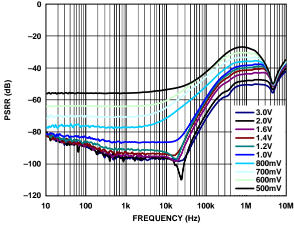
Figure 28. Power Supply Rejection Ratio (PSRR) vs. Frequency, V_{OUT} = 5 V , for Various Headroom Voltages
