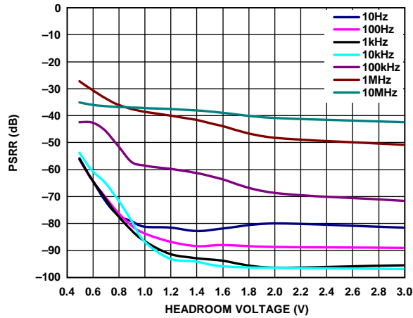
Figure 29. Power Supply Rejection Ratio (PSRR) vs. Headroom Voltage, V_{OUT} = 5 V , for Different Frequencies
