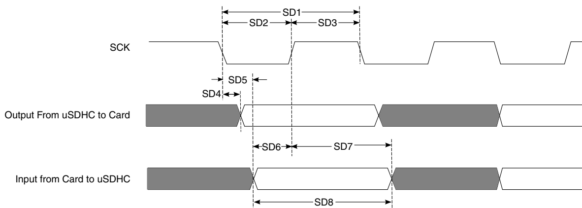
Figure 48. SDR50/SDR104 Timing
