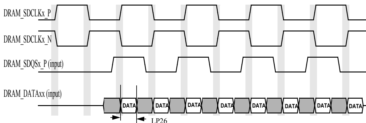
Figure 30. LPDDR2 Read Cycle
