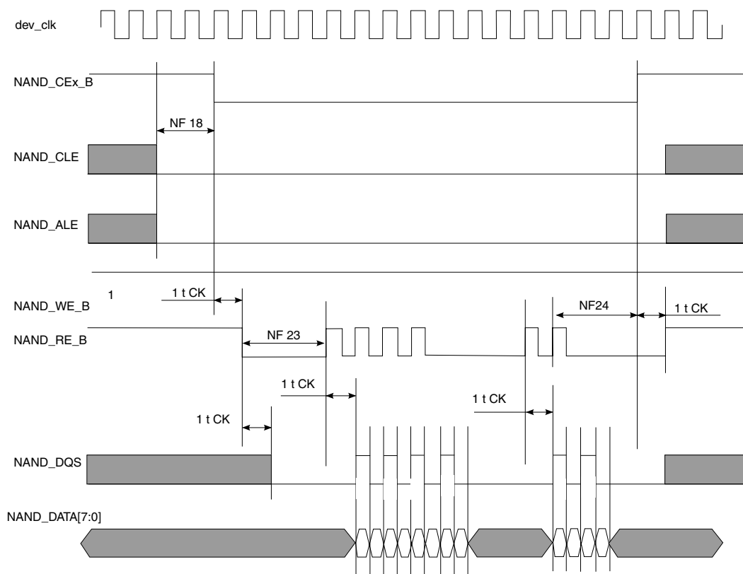
Figure 41. Samsung Toggle Mode Data Read Timing
