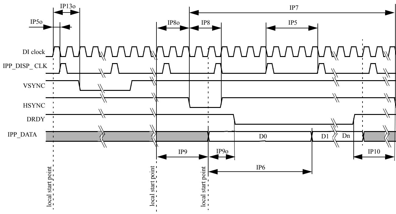
Figure 70. TFT Panels Timing Diagram—Horizontal Sync Pulse
