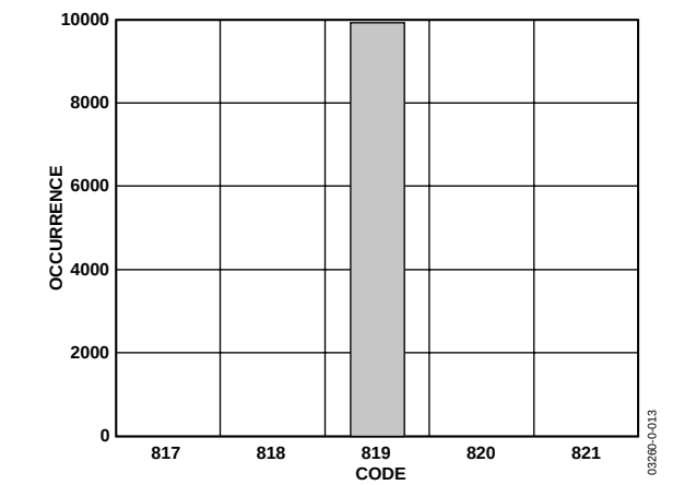
Figure 15. Code Histogram Plot, V_{DD} = 5 V
