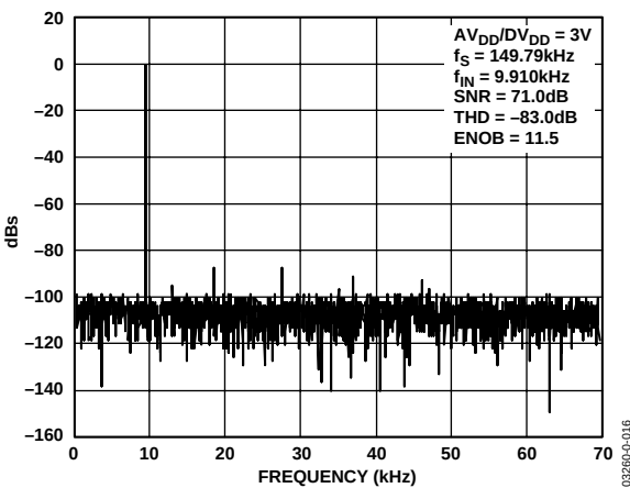
Figure 18. Dynamic Performance at V_{DD} = 3 V
