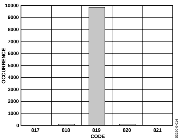
Figure 16. Code Histogram Plot, V_{DD} = 3 V
