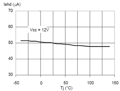
Figure 28. Shutdown current vs. junction temperature
