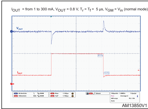
Figure 45. Load transient ( I_{OUT} = 1 to 300 mA, normal mode)
