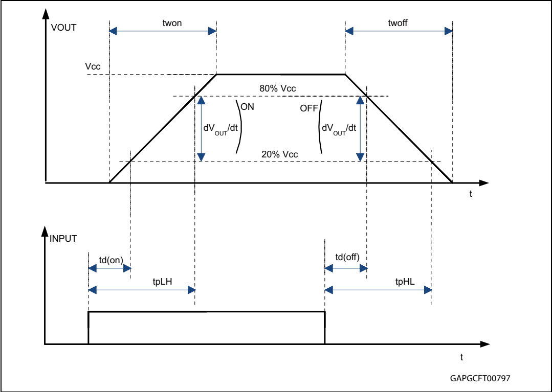
Figure 7. MultiSense timings (current sense mode)
