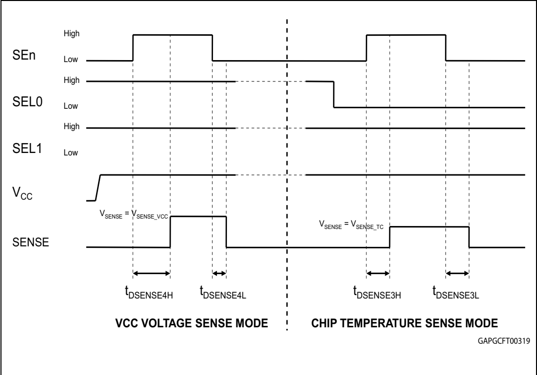
Figure 8. MultiSense timings (chip temperature and V_{CC} sense mode)
