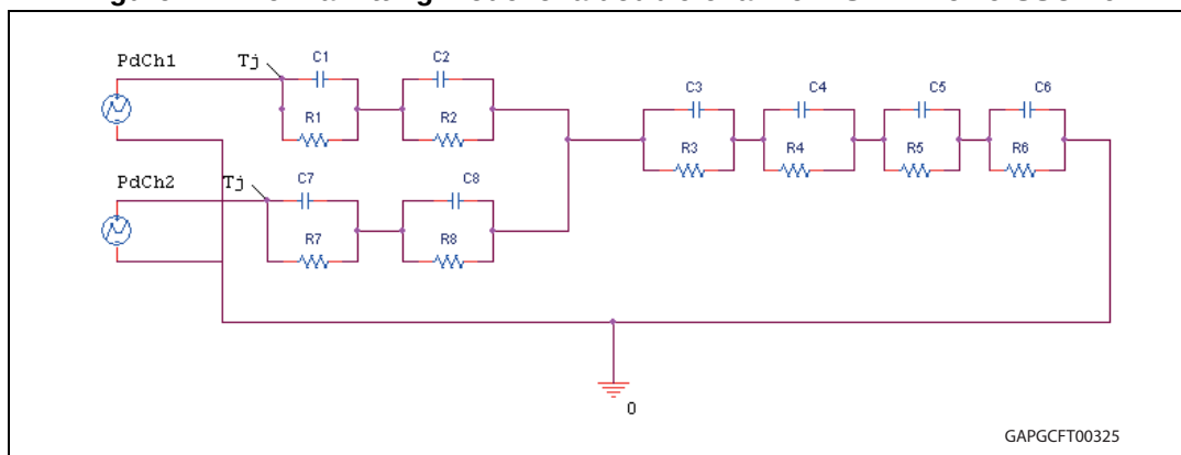
Figure 47. Thermal fitting model of a double-channel HSD in PowerSSO-16
