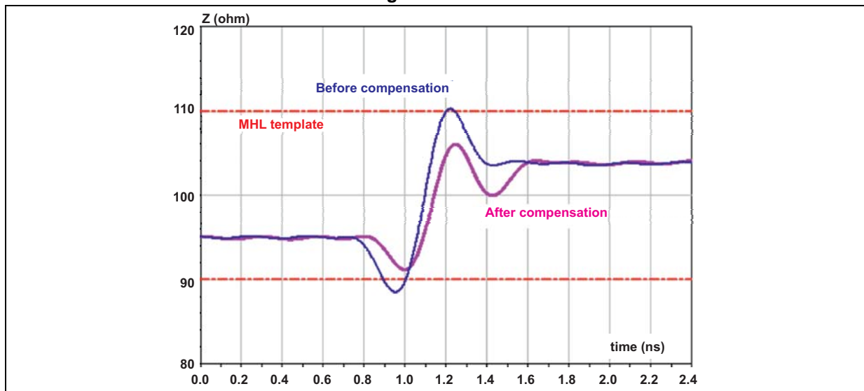
Figure 16. TDR
