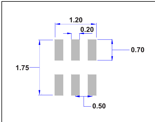
Figure 21. Footprint
