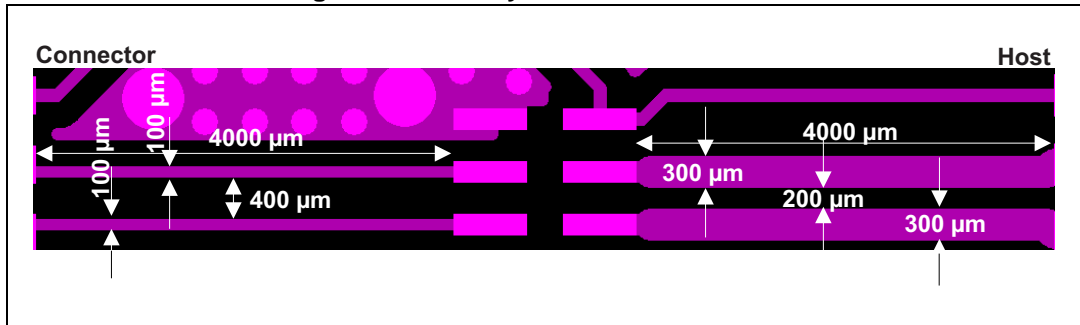
Figure 19. PCB stack dimensions
