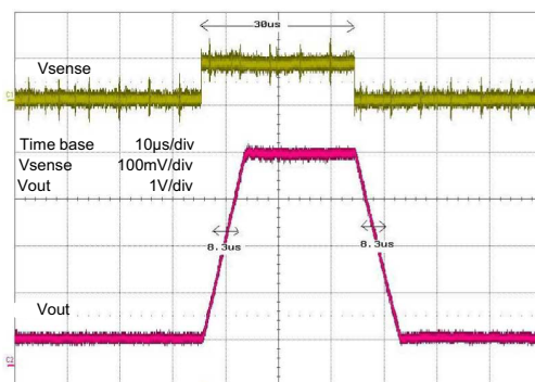
Figure 12. Step response
