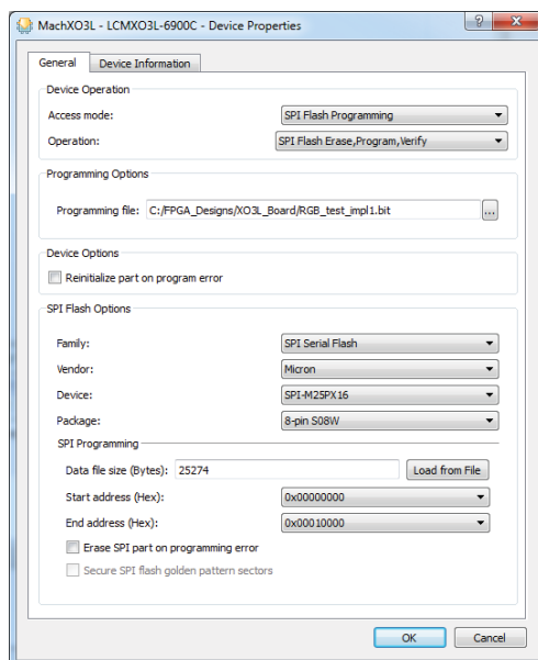
Figure 11. SPI Flash Programming Access Mode
