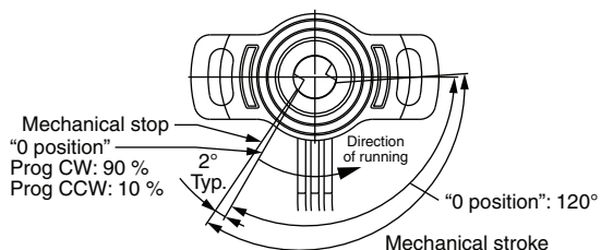
⑤ 981 HE Hollow shaft Spring return CW Shaft: Ø 8 Model: 981HE-2-x-x-W-x-8H00
